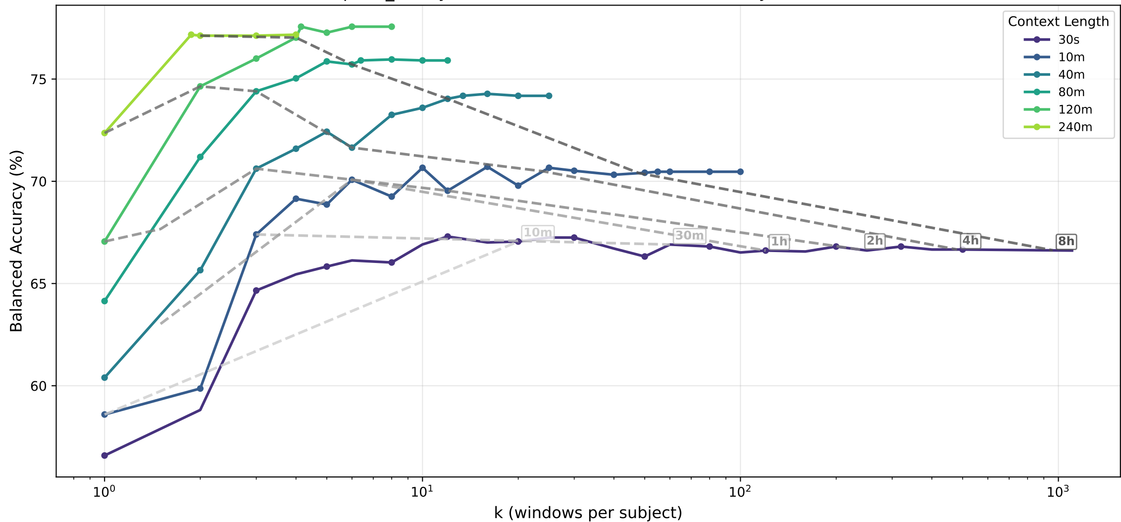
apnea_binary · transformer — Balanced Accuracy (%) vs k
