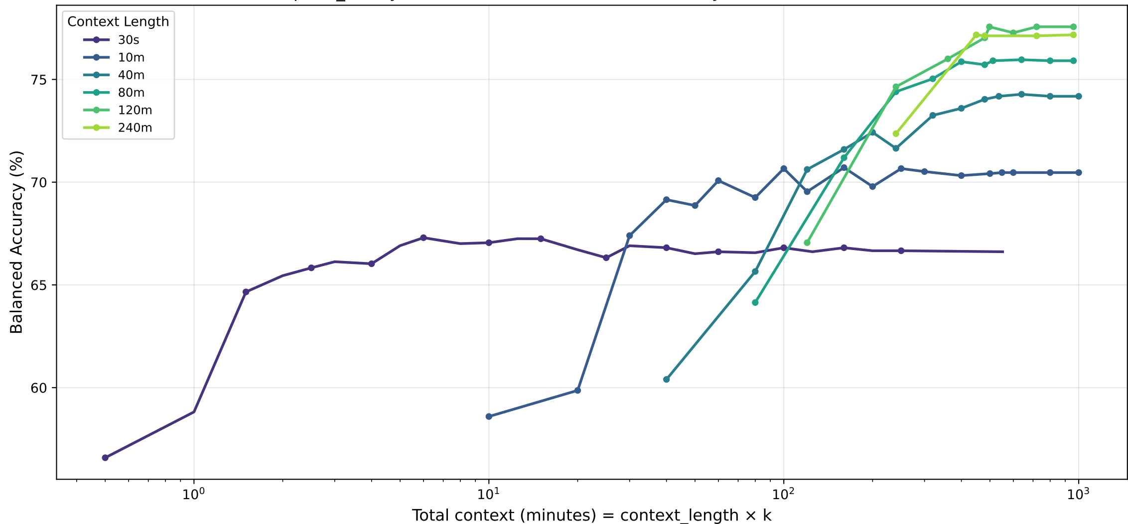
apnea_binary · transformer — Balanced Accuracy (%) vs Total Context
