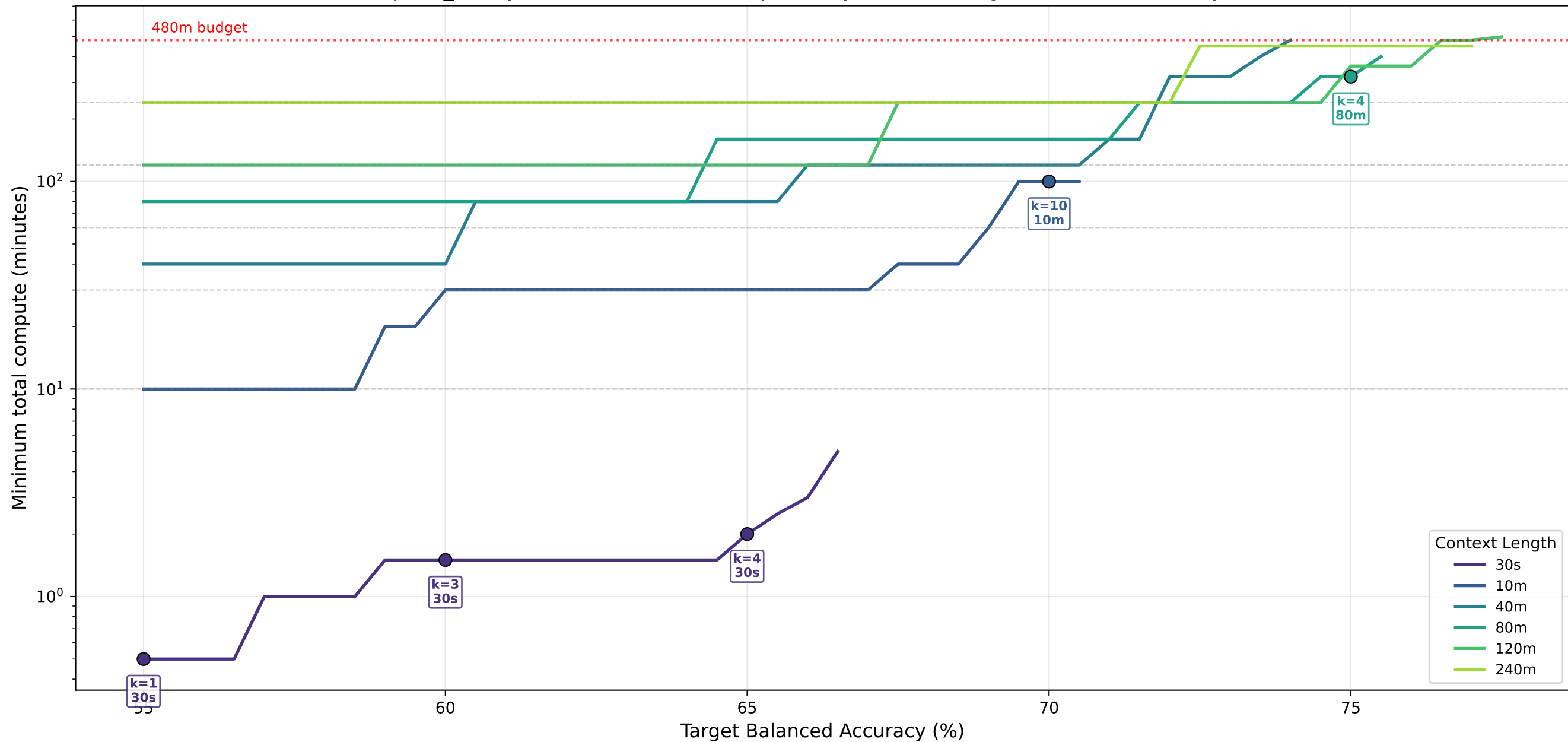
apnea_binary · transformer — Cheapest Way to Reach Target Balanced Accuracy (%)
