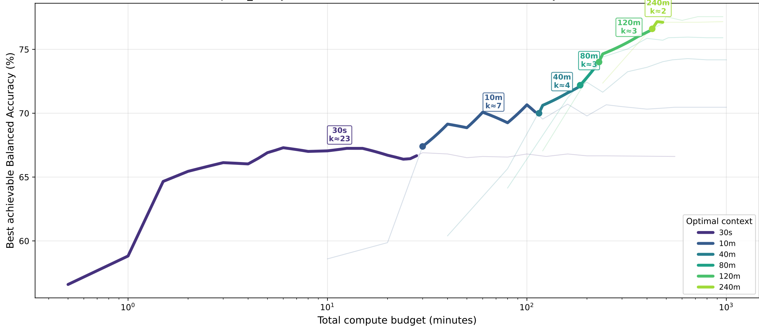
apnea_binary · transformer — Pareto Front: Balanced Accuracy (%)
