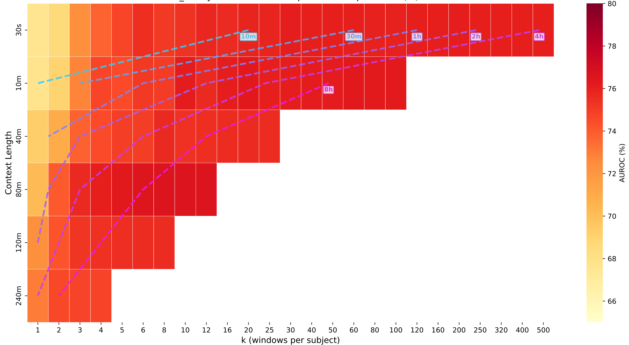
bmi_binary · lstm — Iso-Compute Heatmap: AUROC (%)
