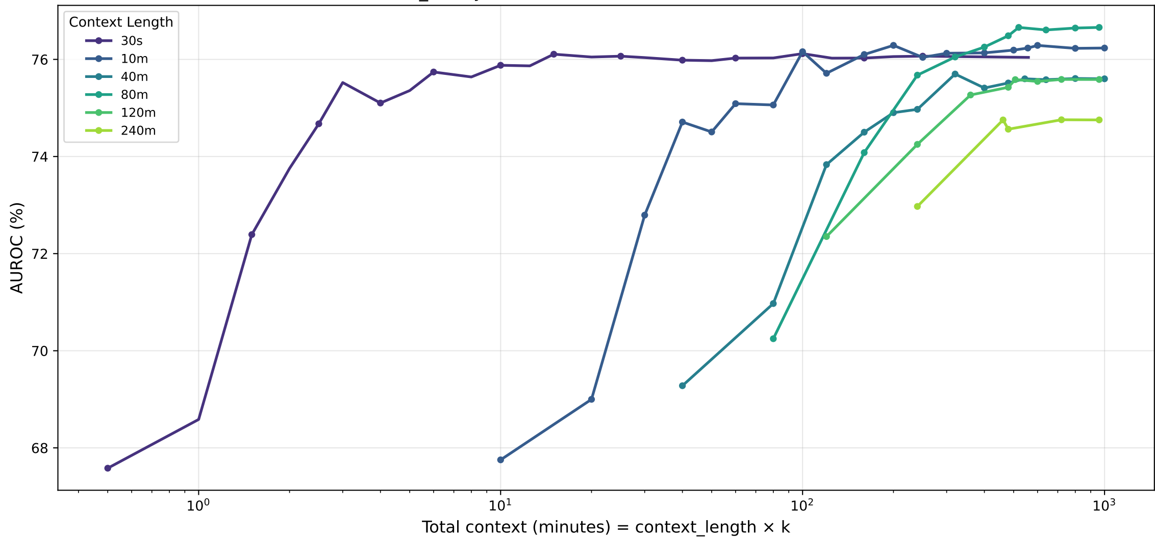
bmi_binary · lstm — AUROC (%) vs Total Context
