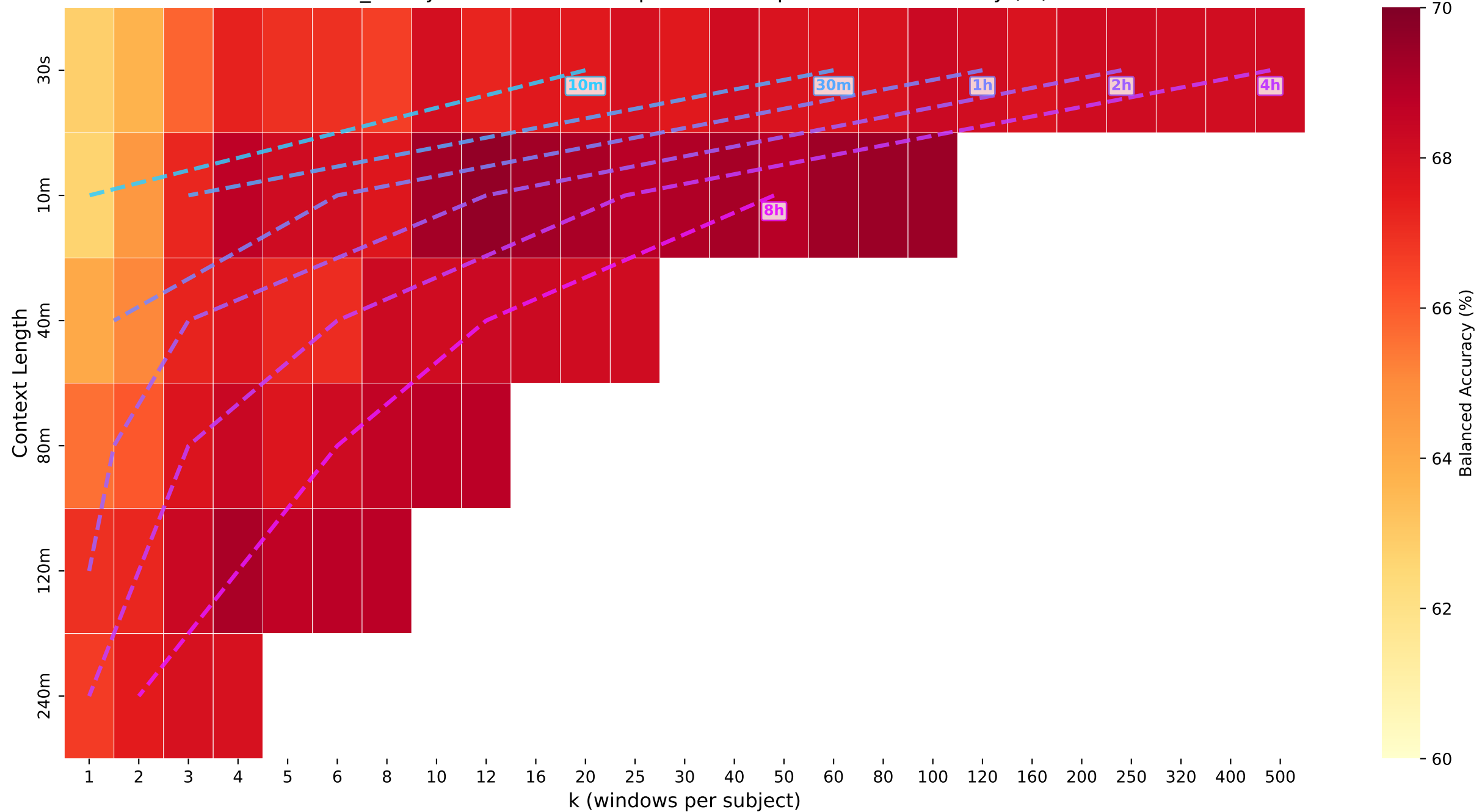
bmi_binary · lstm — Iso-Compute Heatmap: Balanced Accuracy (%)
