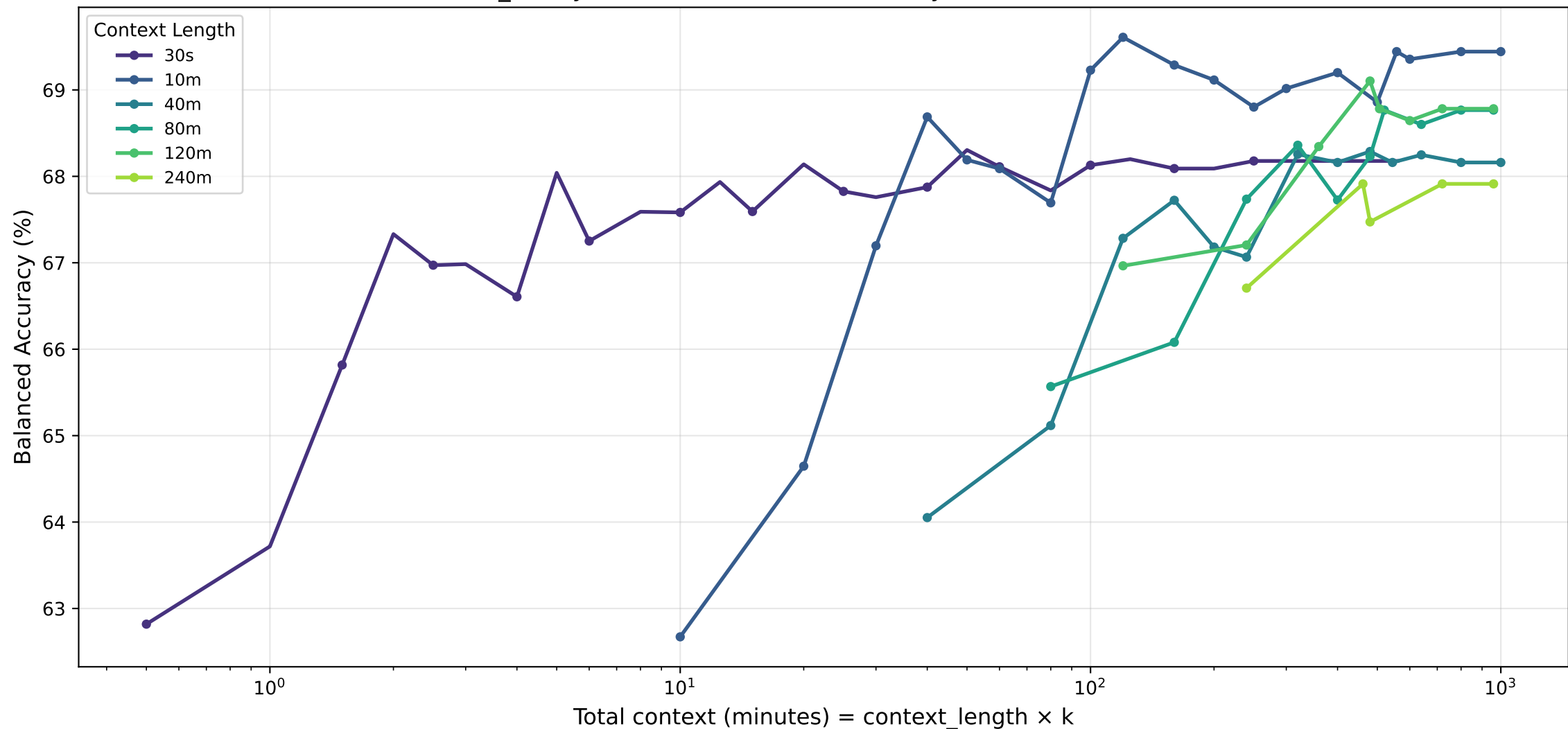
bmi_binary · lstm — Balanced Accuracy (%) vs Total Context
