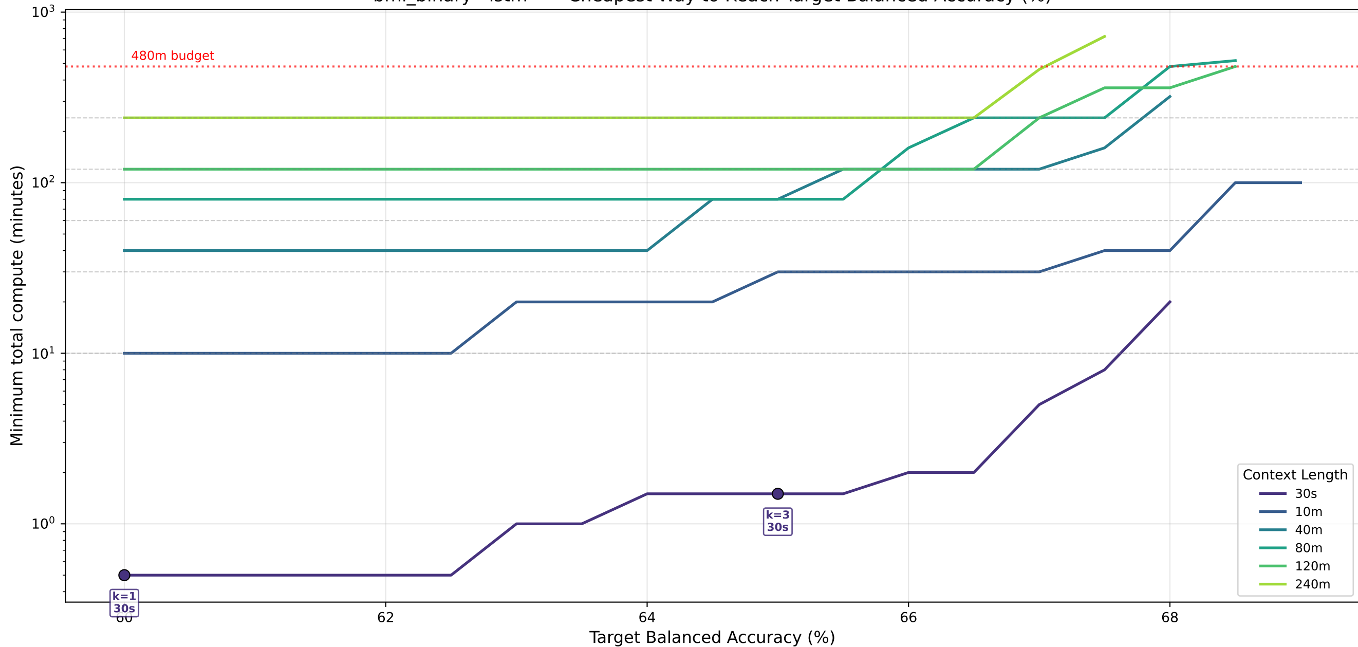
bmi_binary · lstm — Cheapest Way to Reach Target Balanced Accuracy (%)
