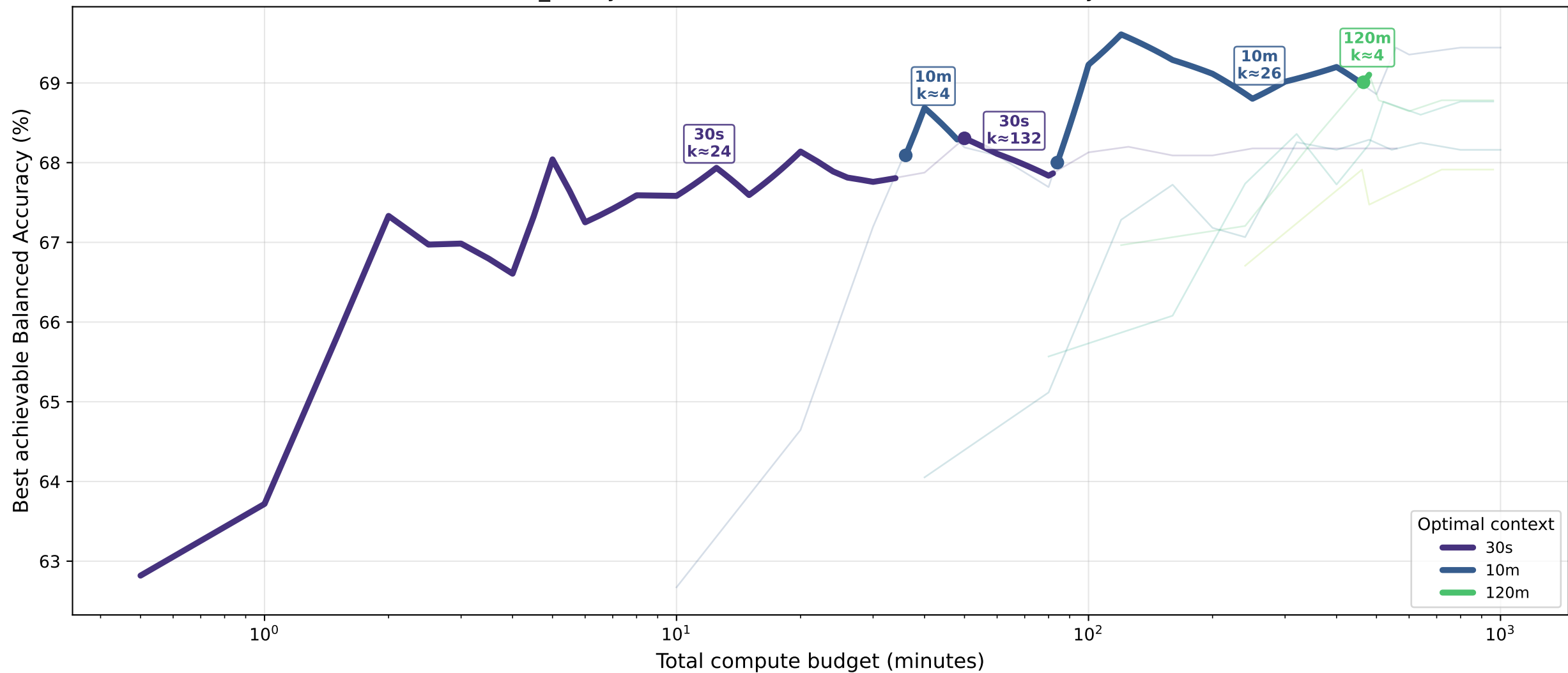
bmi_binary · lstm — Pareto Front: Balanced Accuracy (%)
