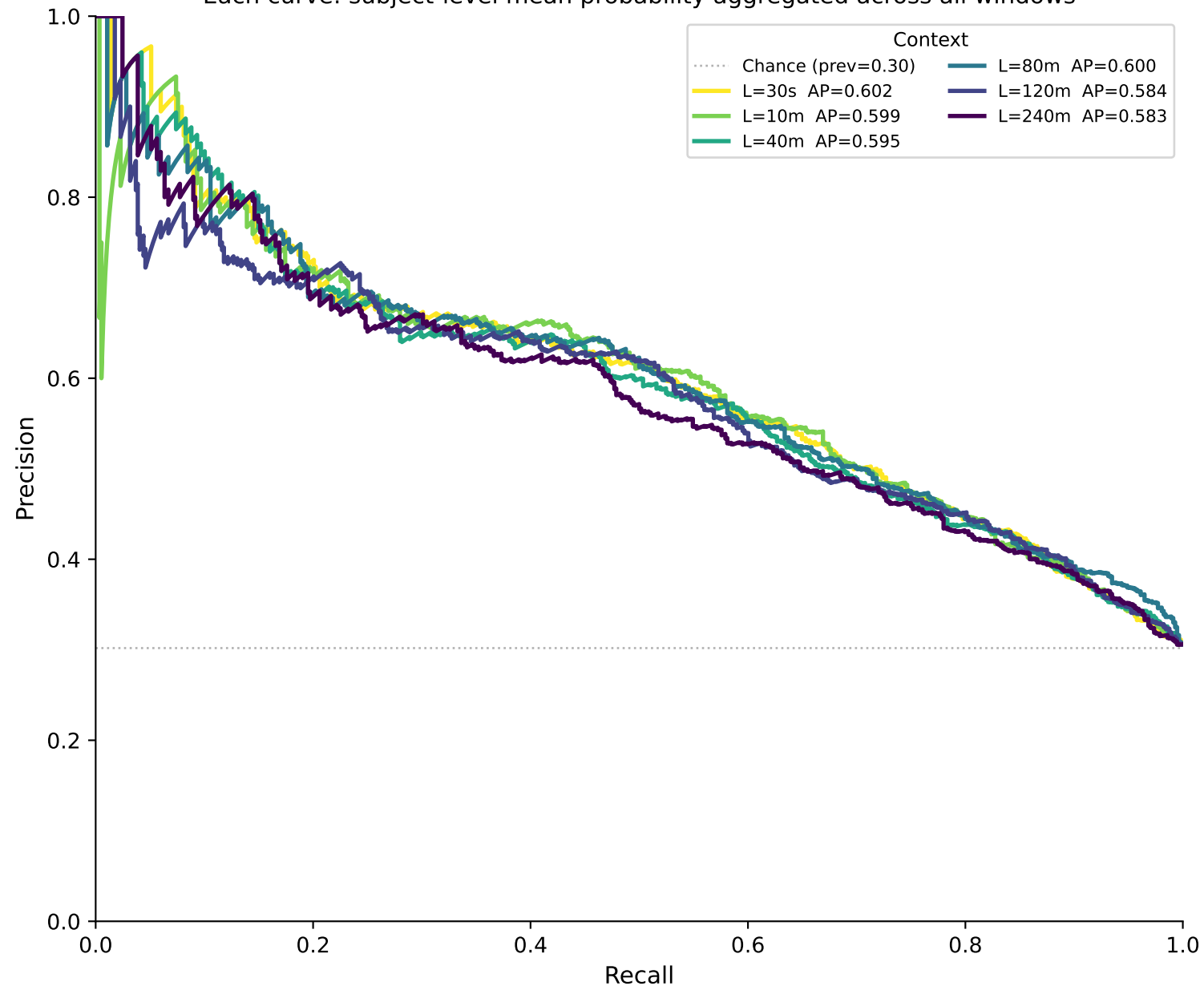
Precision-Recall Curves — bmi_binary (LSTM) K=all Each curve: subject-level mean probability aggregated across all windows
