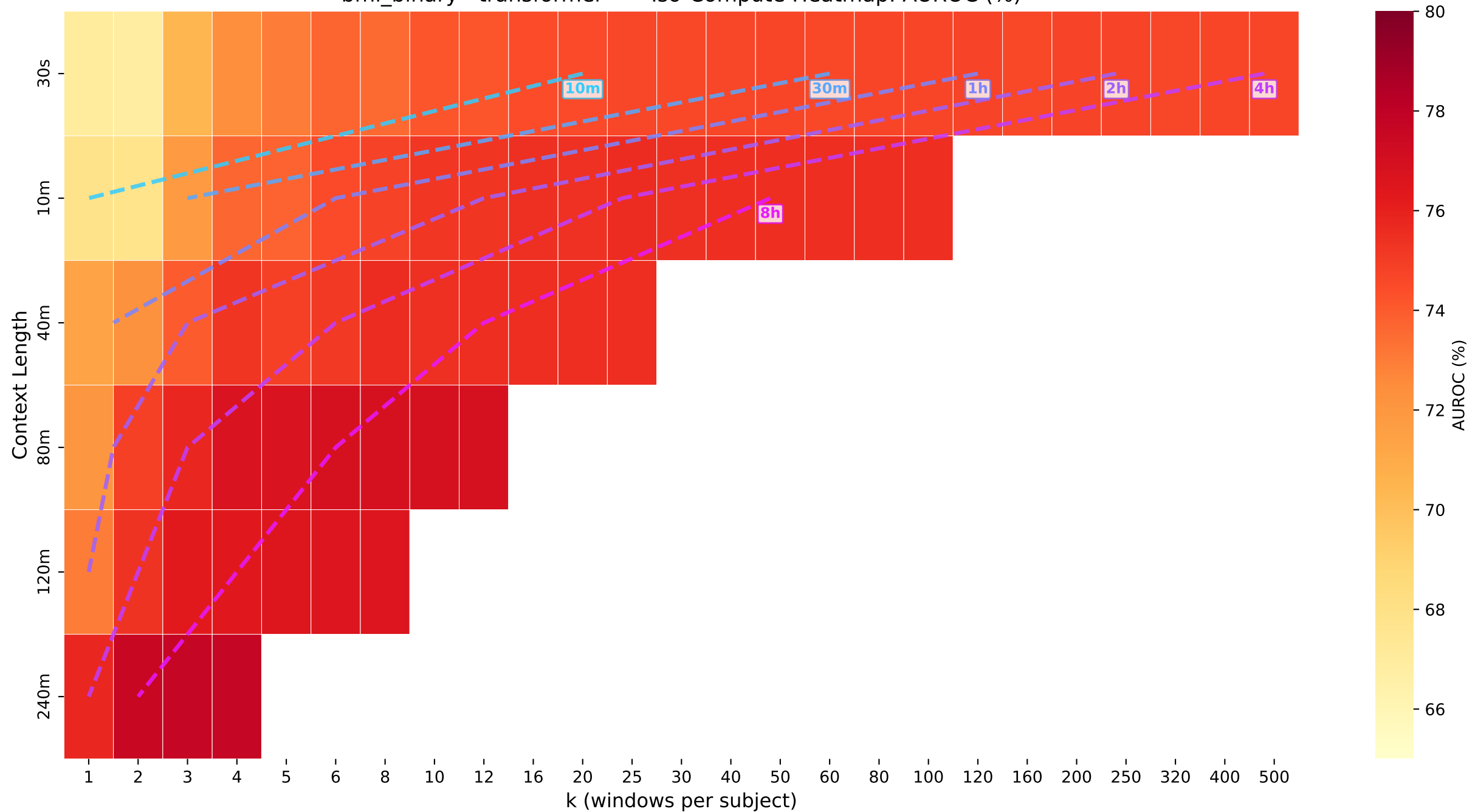
bmi_binary · transformer — Iso-Compute Heatmap: AUROC (%)
