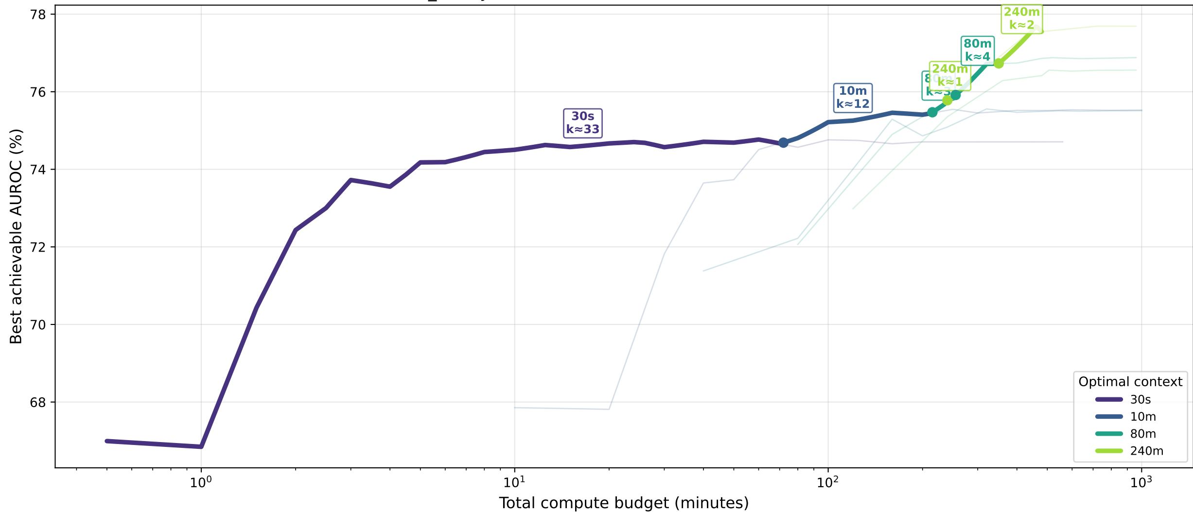
bmi_binary · transformer — Pareto Front: AUROC (%)
