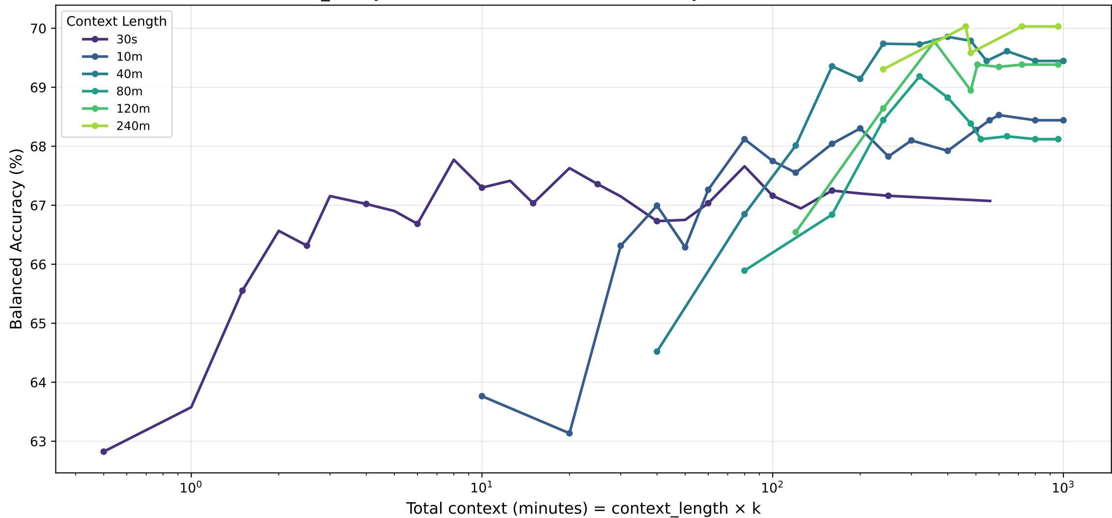
bmi_binary · transformer — Balanced Accuracy (%) vs Total Context
