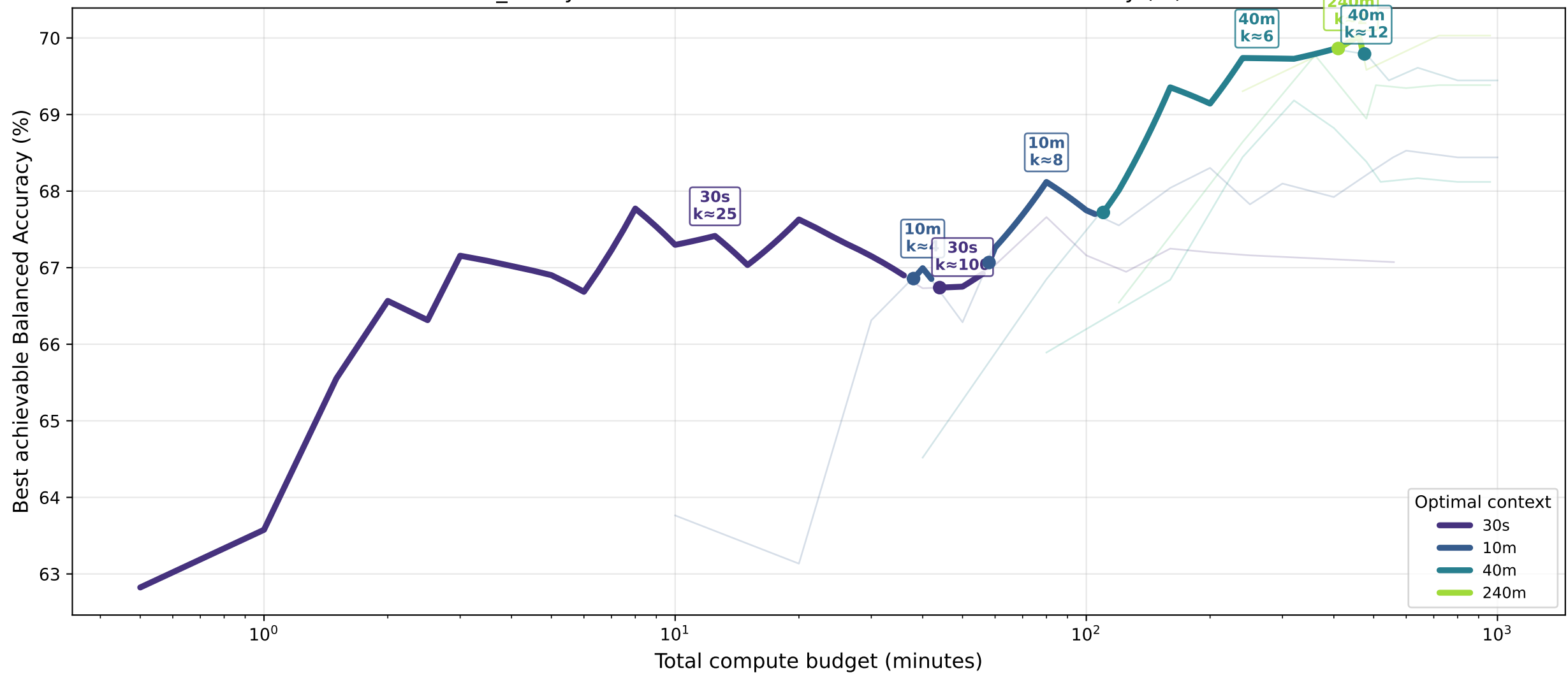
bmi_binary · transformer — Pareto Front: Balanced Accuracy (%)
