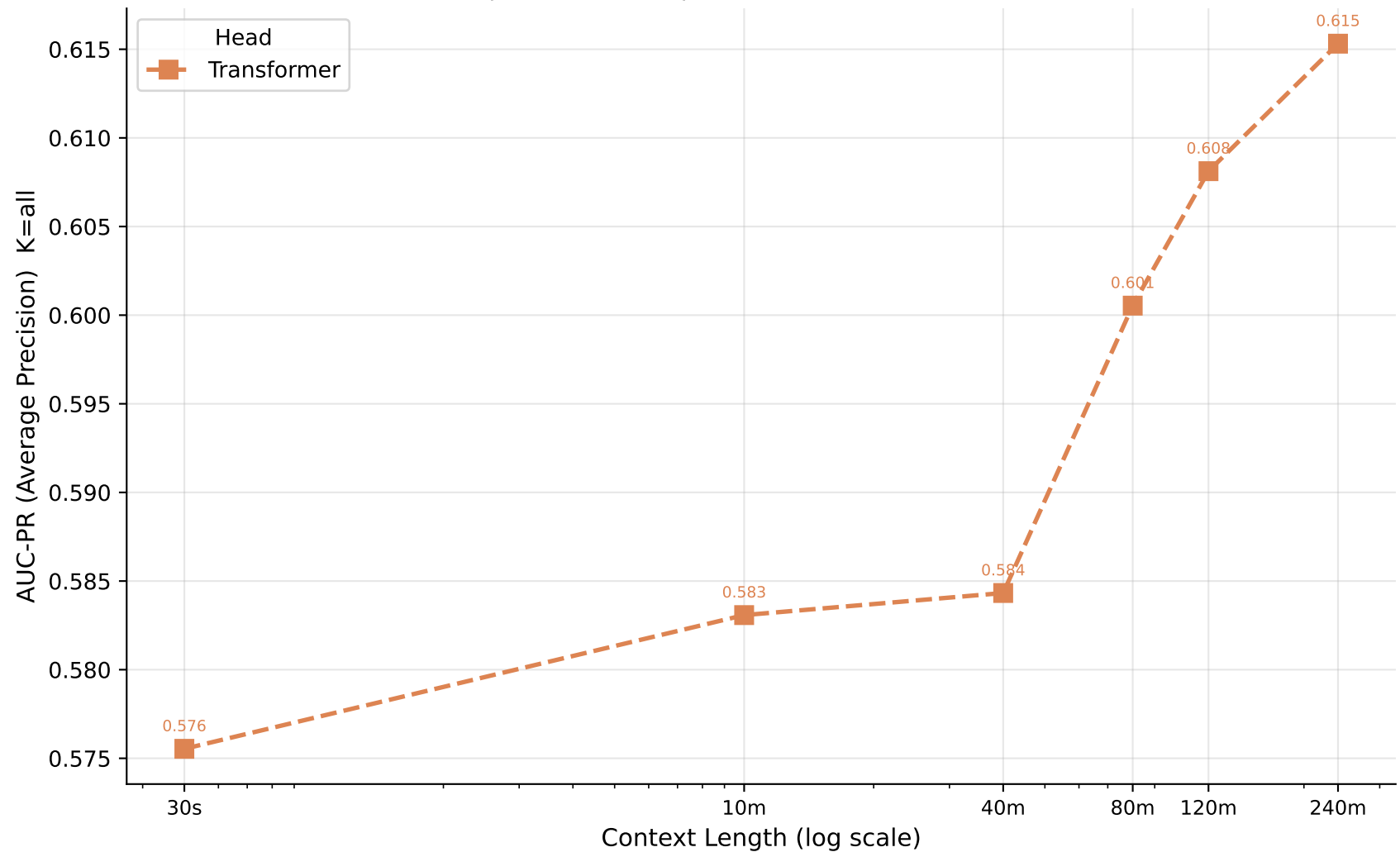
AUC-PR vs Context Length — bmi_binary Does precision-recall performance saturate like AUROC?
