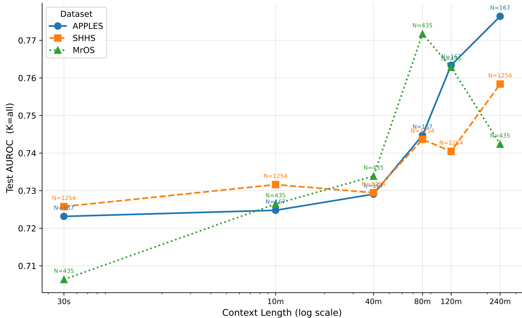
Cohort-Stratified Saturation — bmi_binary (TRANSFORMER) Does the context saturation result hold across each dataset independently?
