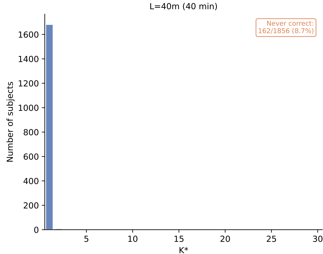
K* Distribution — bmi_binary (TRANSFORMER) K* = minimum windows for correct classification (reps=20)
