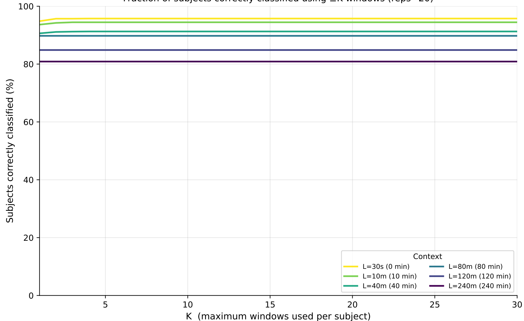
Coverage Curves — bmi_binary (TRANSFORMER) Fraction of subjects correctly classified using \leq K windows (reps=20)
