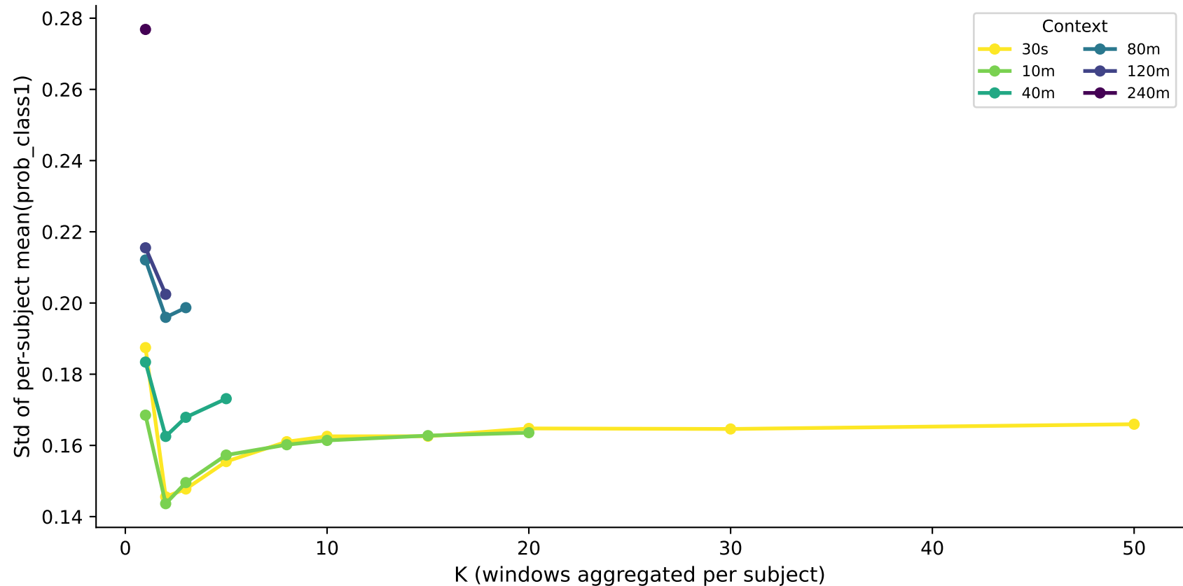
Prediction Variance vs K — bmi_binary (TRANSFORMER) Aggregation stabilises predictions (lower std = more consistent)
