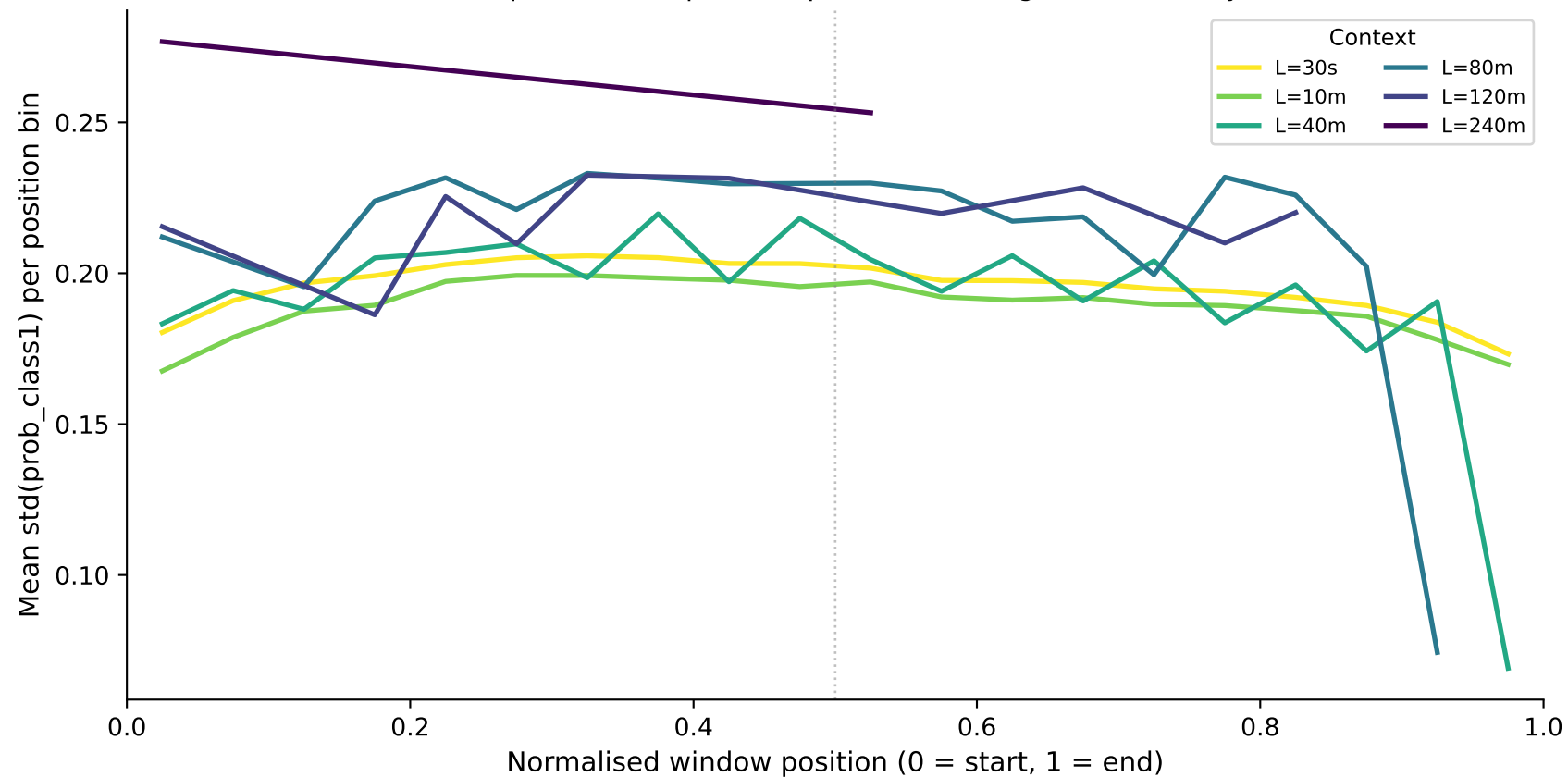
Prediction Variance vs Night Position — bmi_binary (TRANSFORMER) Lower variance = position-independent predictions (longer context may flatten this)
