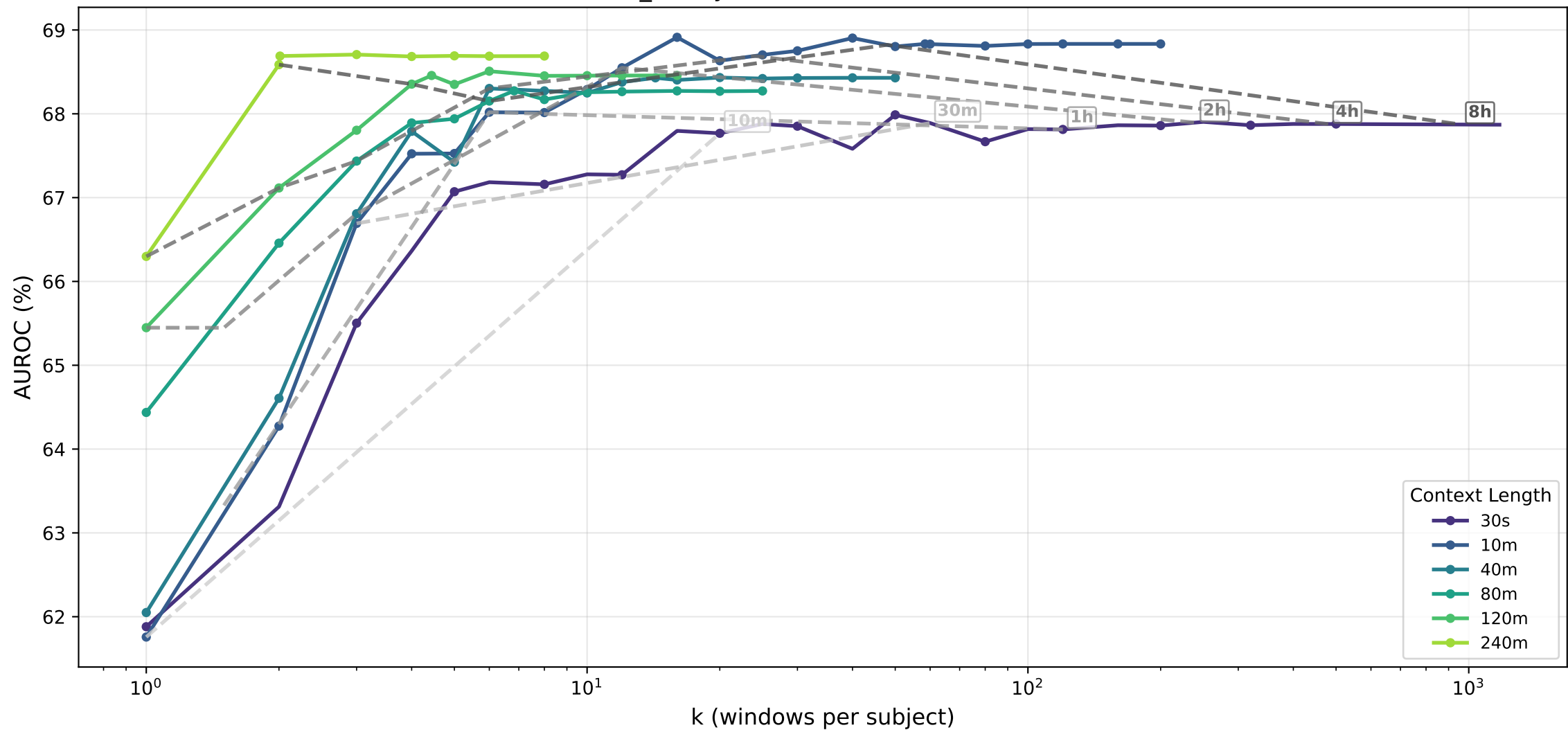
cvd_binary · lstm — AUROC (%) vs k
