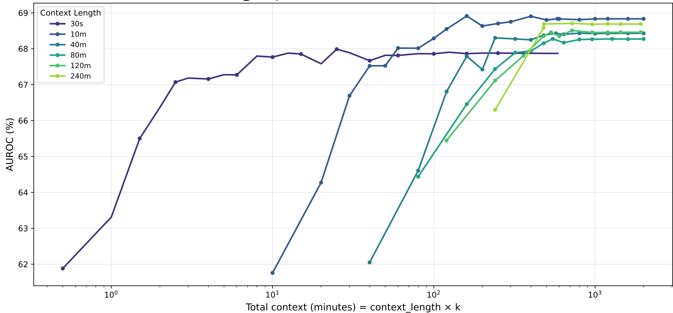
cvd_binary · lstm — AUROC (%) vs Total Context
