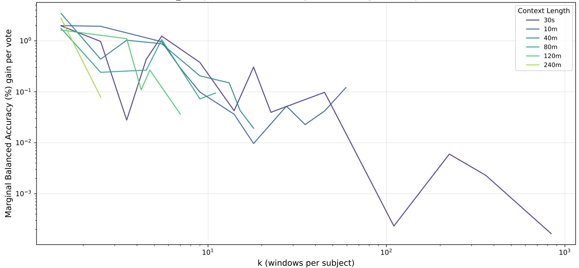
cvd_binary · Istm — Diminishing Returns: Marginal Gain per Vote
