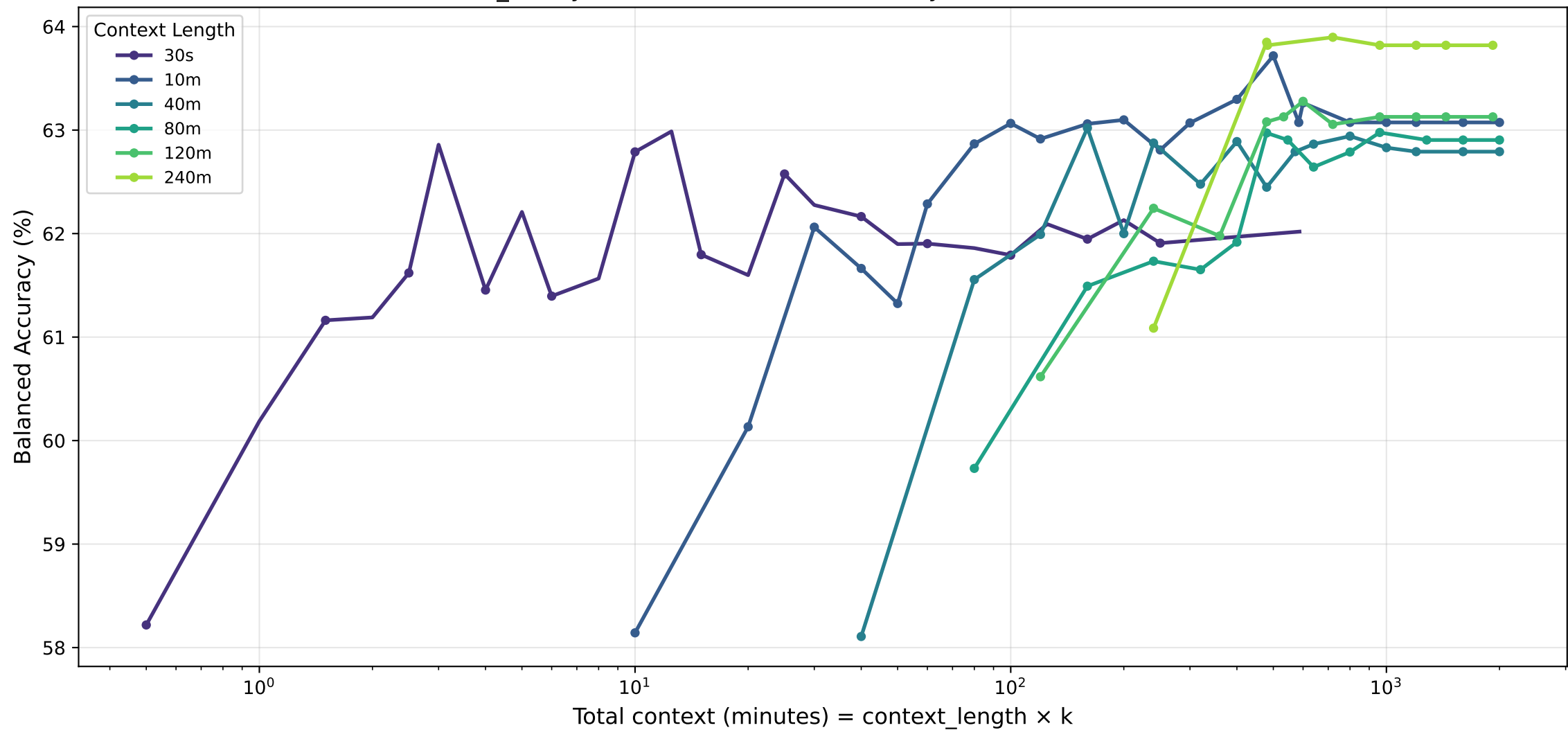
cvd_binary · lstm — Balanced Accuracy (%) vs Total Context
