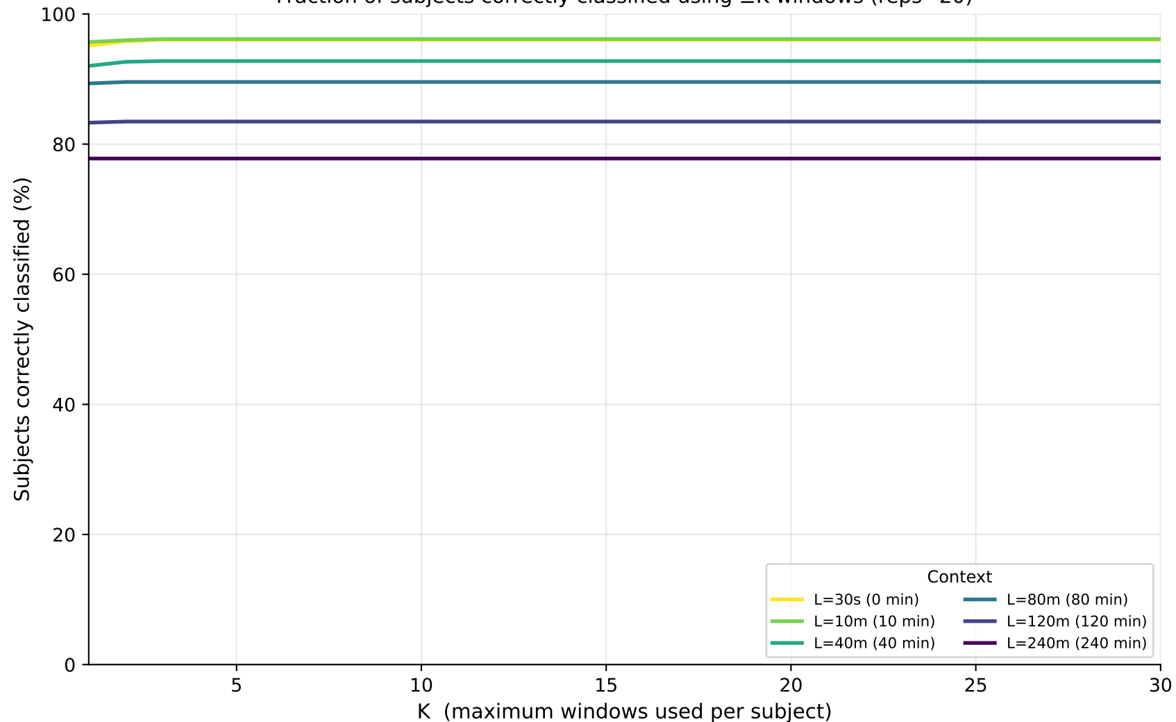
Coverage Curves — cvd_binary (LSTM) Fraction of subjects correctly classified using \leq K windows (reps=20)
