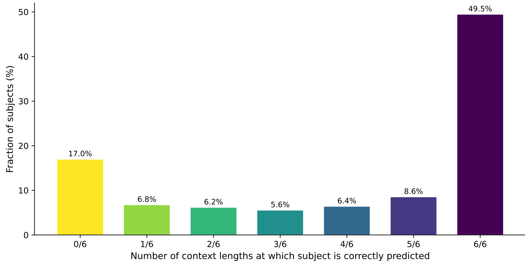
Hard-Subject Analysis — cvd_binary (LSTM) N = 1742 subjects · 0/6 = never correct (irreducible hard cases)
