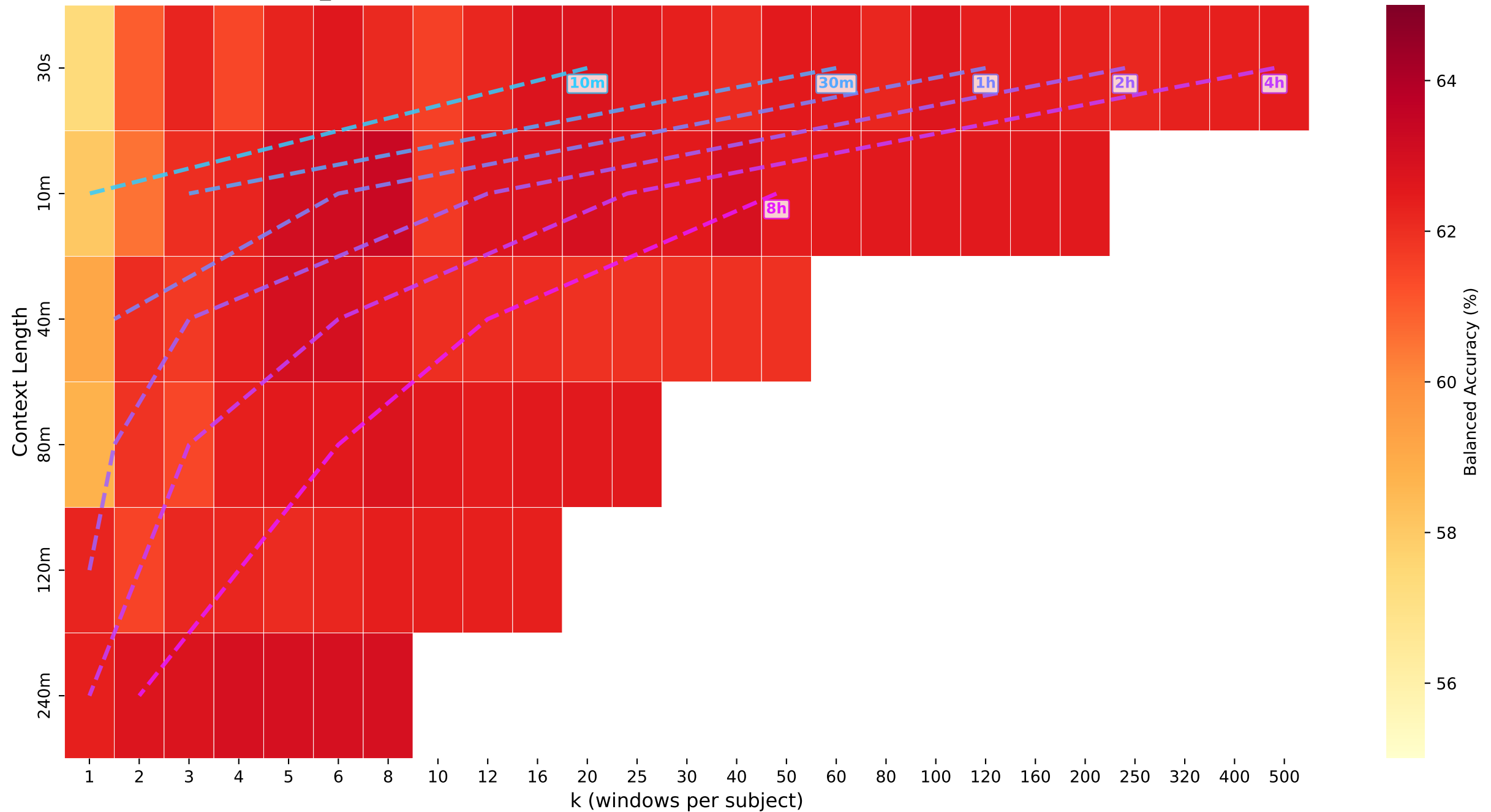
cvd_binary · transformer — Iso-Compute Heatmap: Balanced Accuracy (%)
