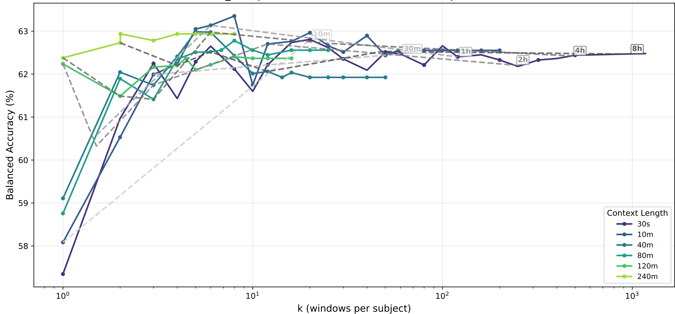
cvd_binary · transformer — Balanced Accuracy (%) vs k
