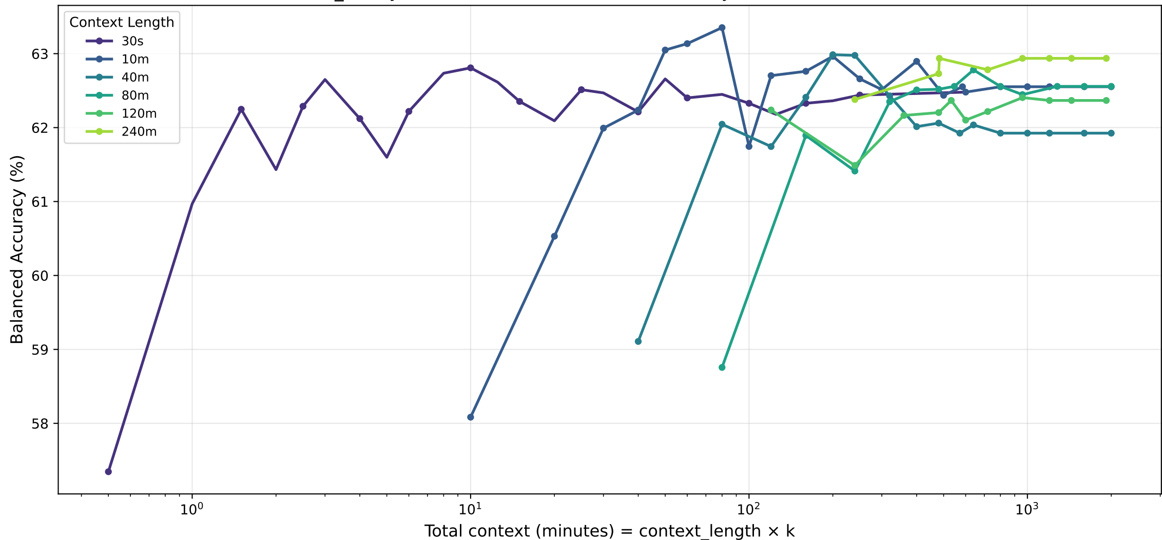
cvd_binary · transformer — Balanced Accuracy (%) vs Total Context
