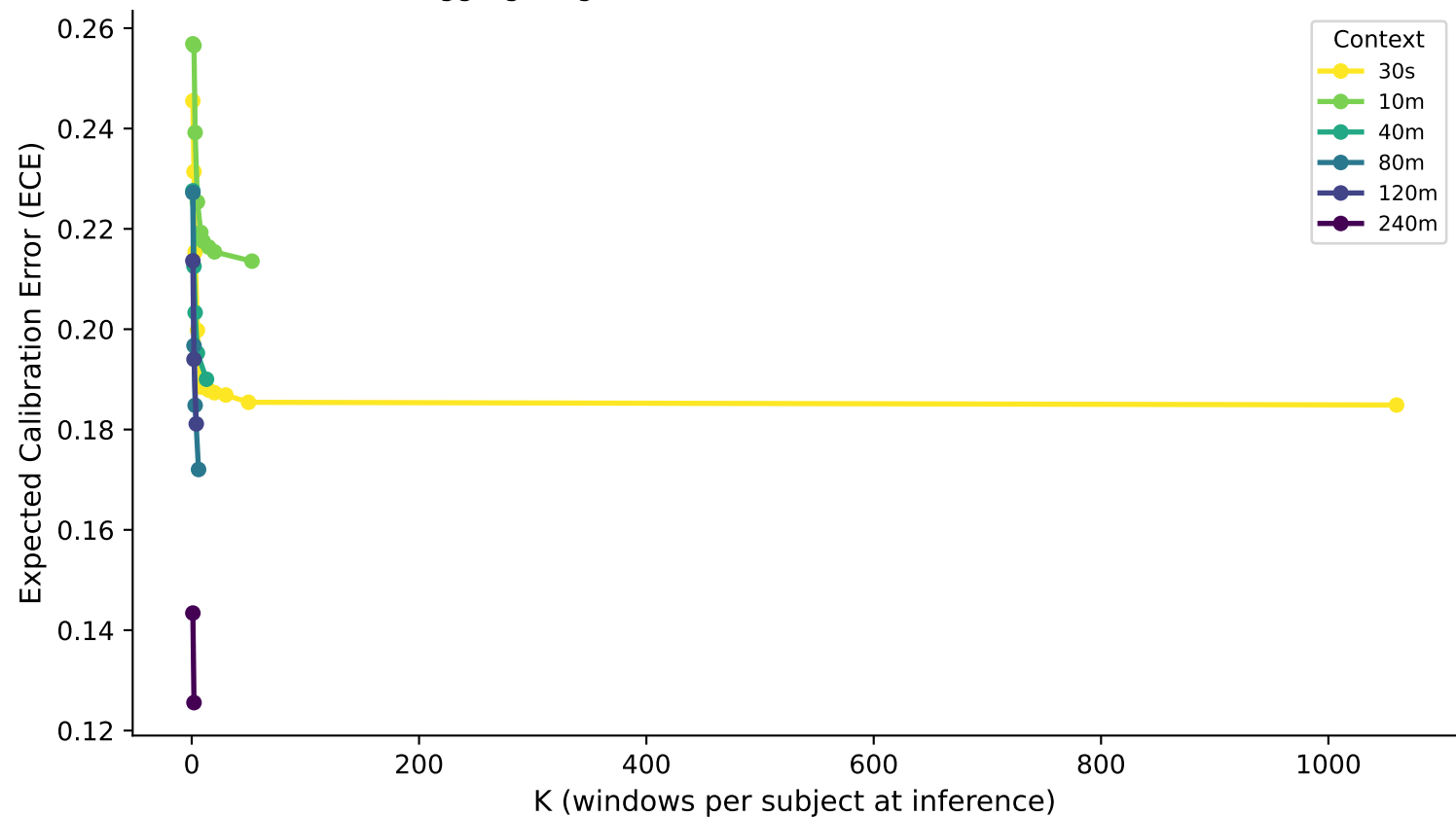
ECE vs K — cvd_binary (TRANSFORMER) Aggregating more windows reduces calibration error
