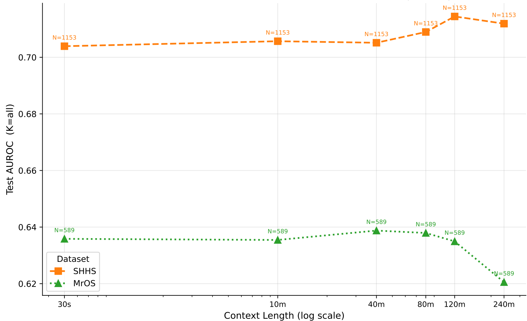
Cohort-Stratified Saturation — cvd_binary (TRANSFORMER) Does the context saturation result hold across each dataset independently?
