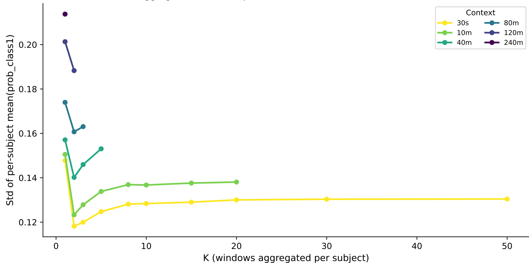
Prediction Variance vs K — cvd_binary (TRANSFORMER) Aggregation stabilises predictions (lower std = more consistent)
