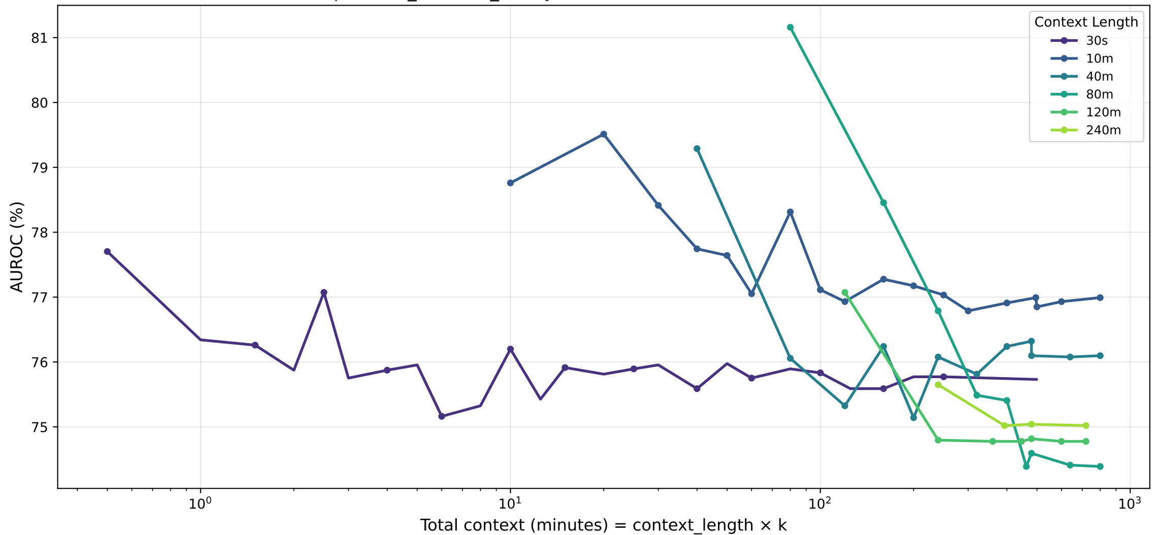
depression_extreme_binary · lstm — AUROC (%) vs Total Context
