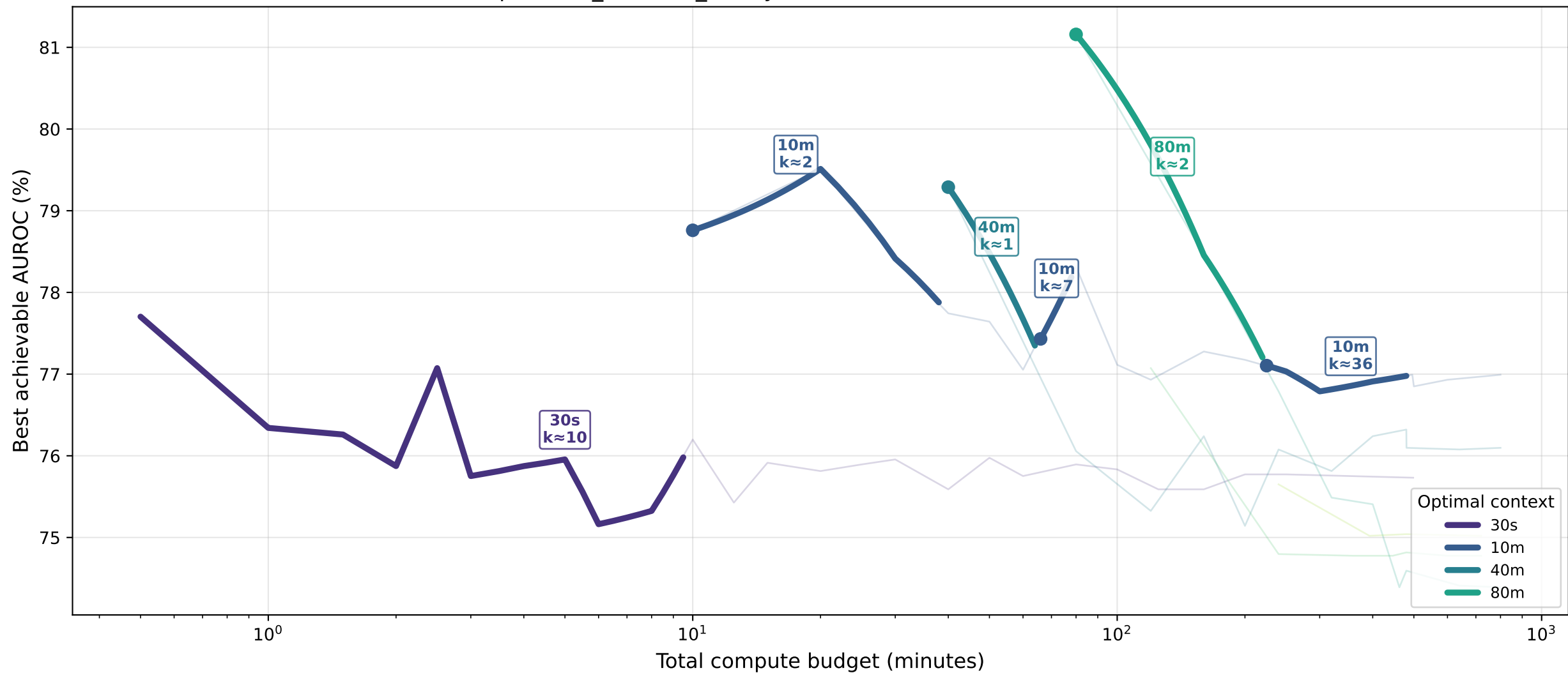
depression_extreme_binary · lstm — Pareto Front: AUROC (%)
