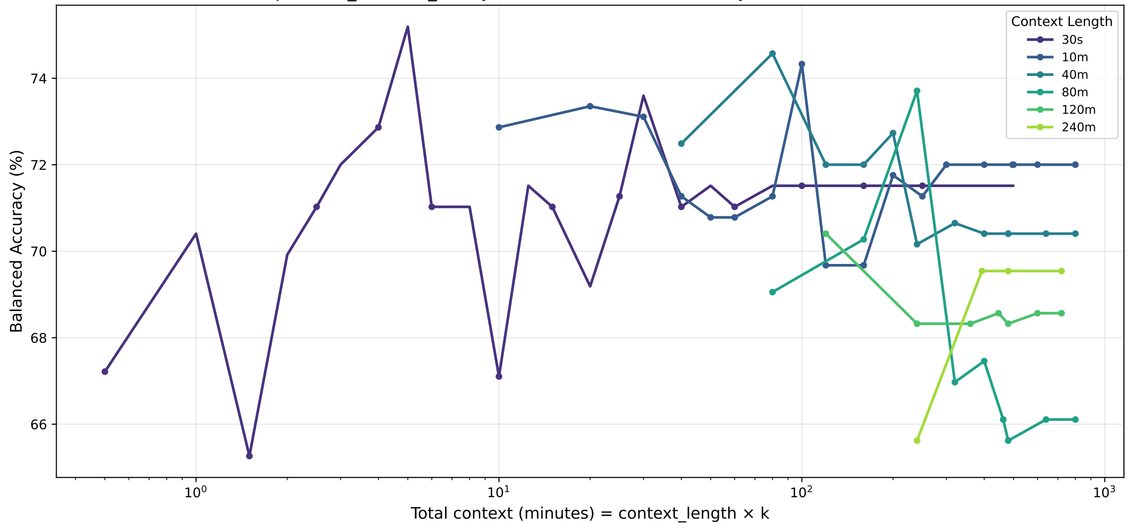
depression_extreme_binary · lstm — Balanced Accuracy (%) vs Total Context
