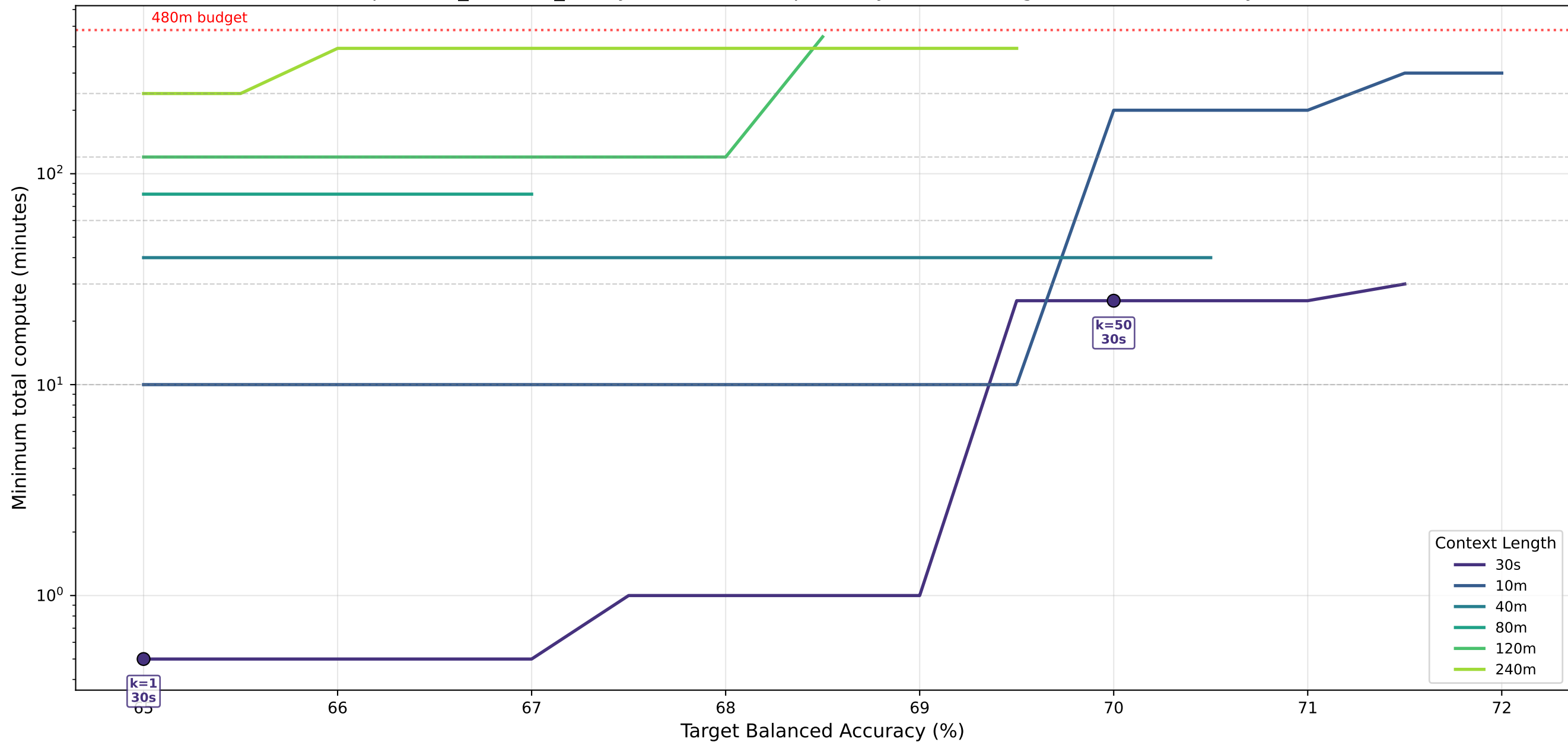
depression_extreme_binary · lstm — Cheapest Way to Reach Target Balanced Accuracy (%)
