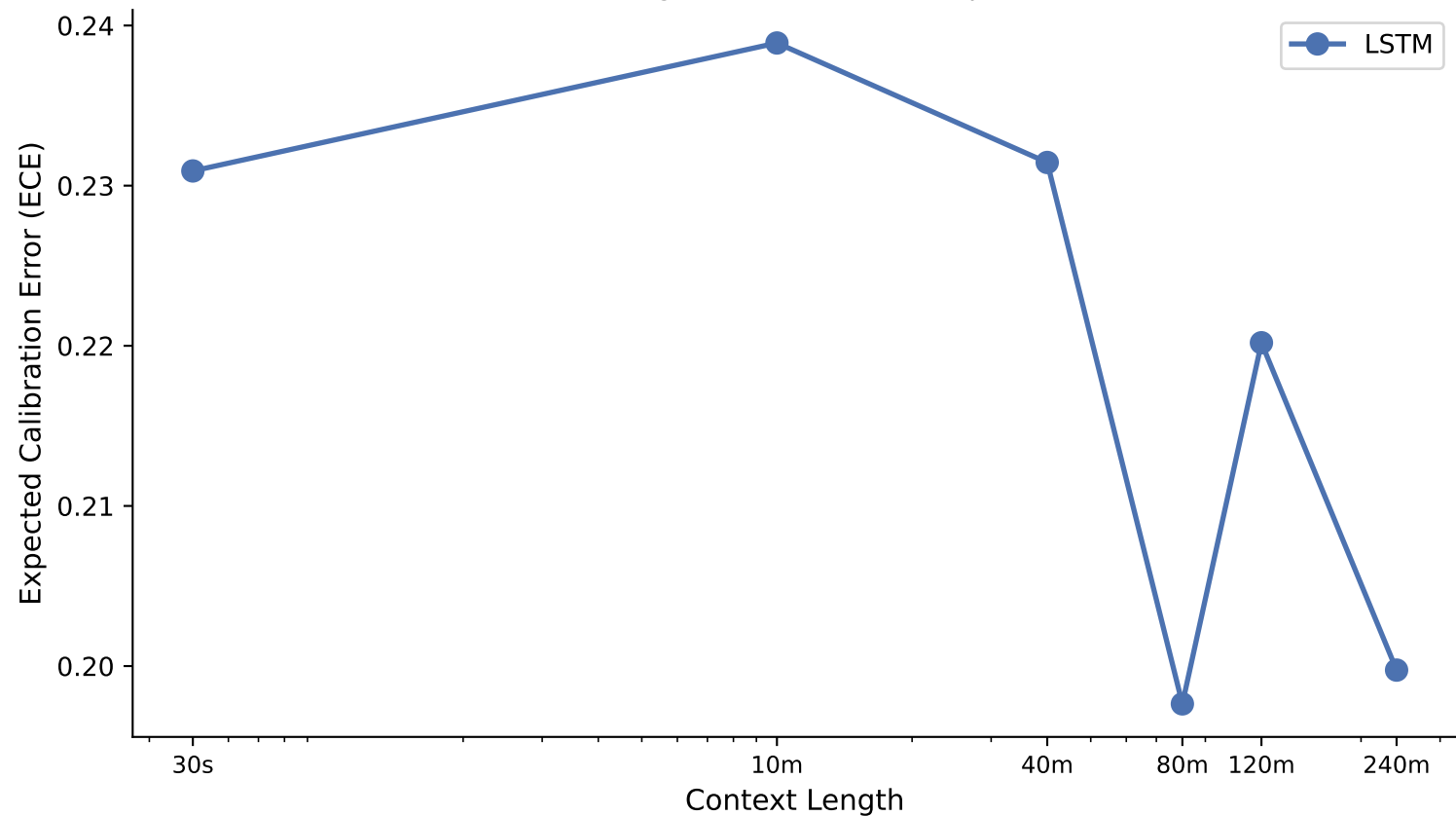
ECE vs Context Length — depression_extreme_binary (K=10) Lower is better; longer context should improve calibration
