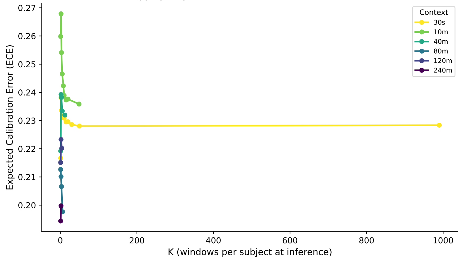
ECE vs K — depression_extreme_binary (LSTM) Aggregating more windows reduces calibration error
