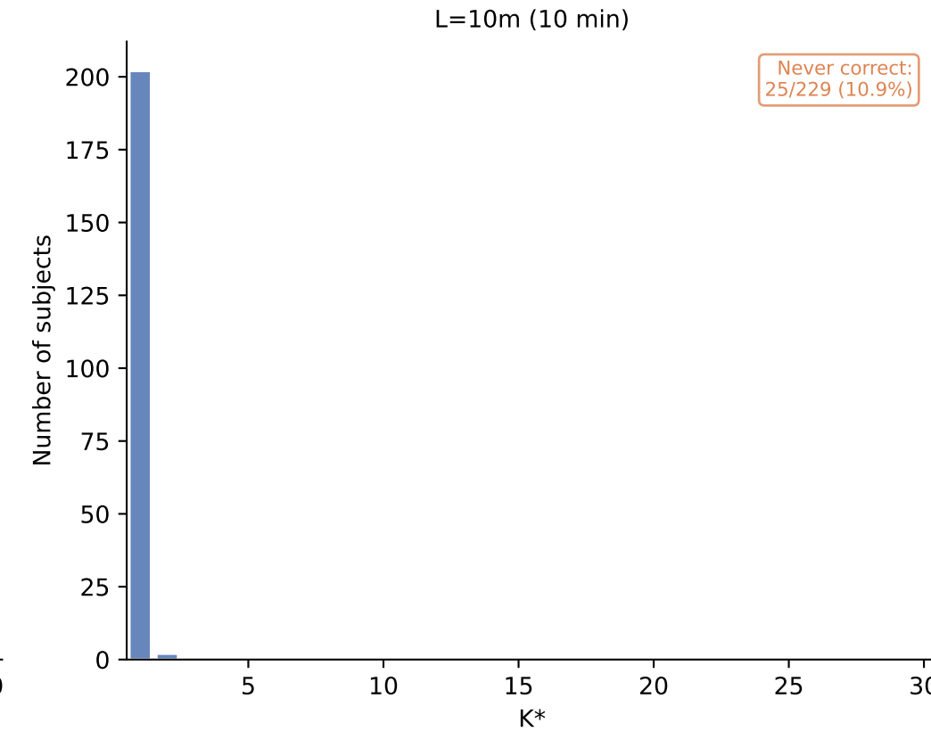
K* Distribution — depression_extreme_binary (LSTM) K* = minimum windows for correct classification (reps=20)
