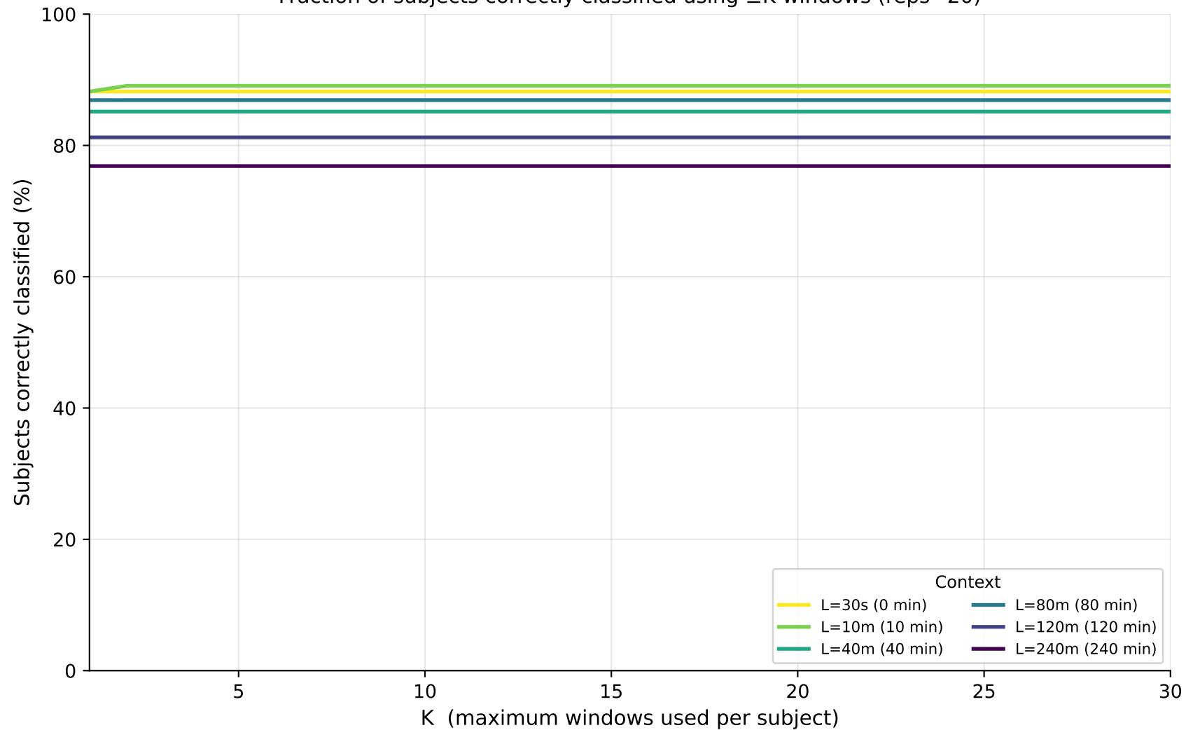
Coverage Curves — depression_extreme_binary (LSTM) Fraction of subjects correctly classified using \leq K windows (reps=20)
