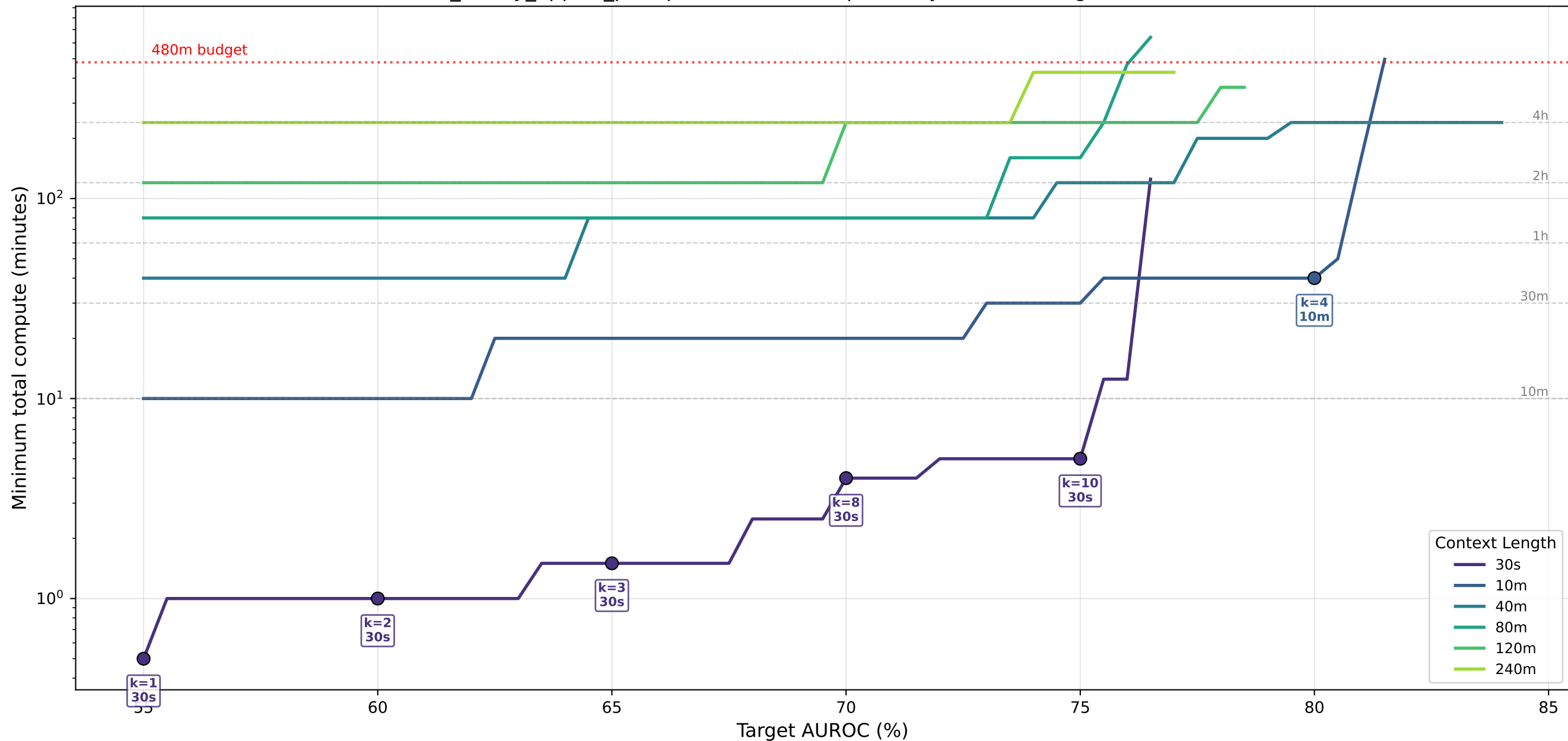
osa_binary_apples_postqc · lstm — Cheapest Way to Reach Target AUROC (%)
