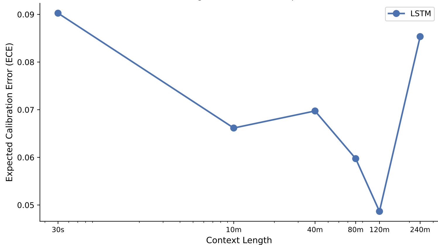
ECE vs Context Length — osa_binary_apples_postqc (K=10) Lower is better; longer context should improve calibration
