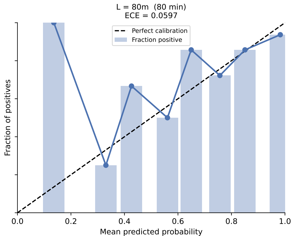
Reliability Diagrams — osa_binary_apples_postqc (LSTM, K=10) Diagonal = perfect calibration
