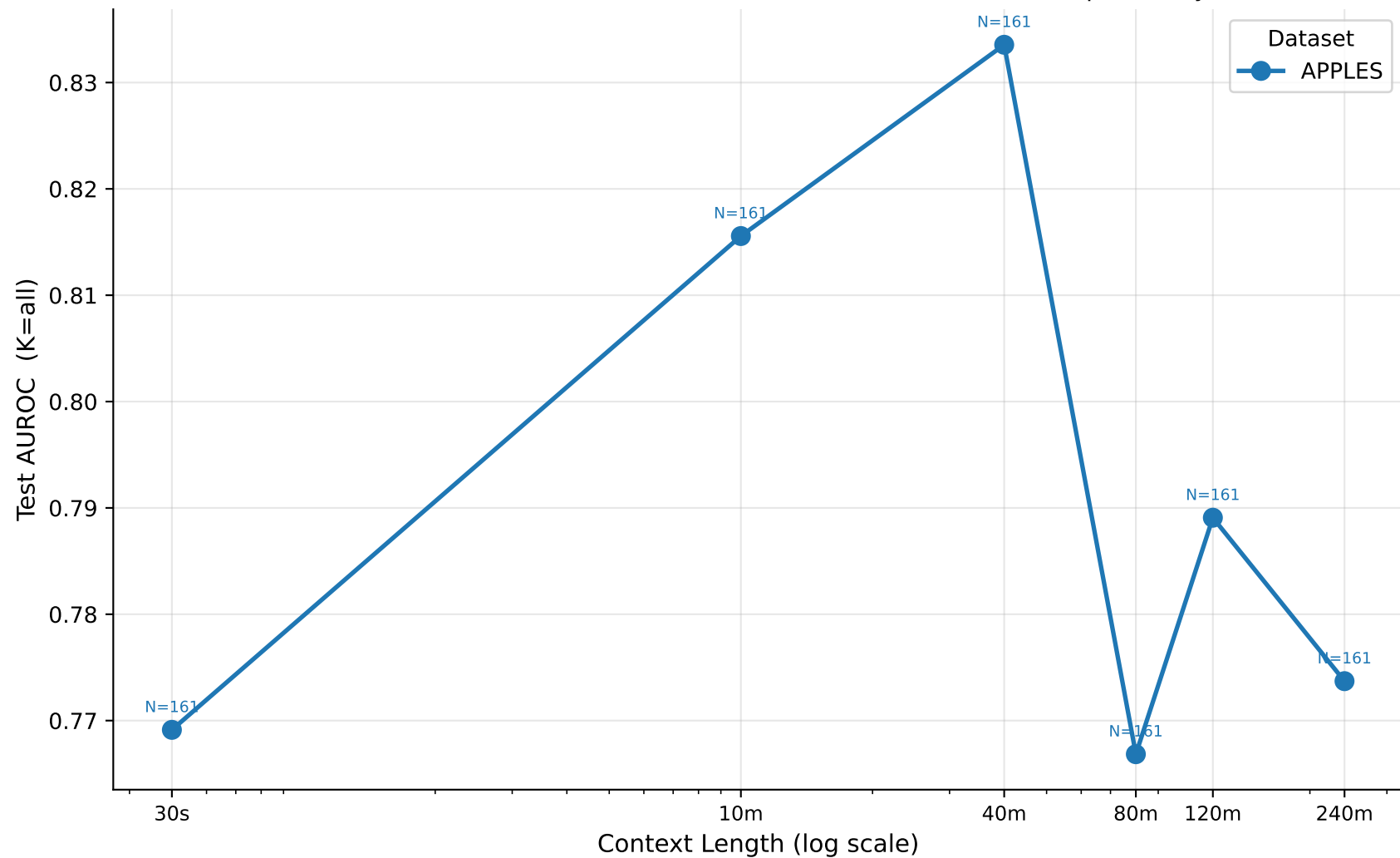
Cohort-Stratified Saturation — osa_binary_apples_postqc (LSTM) Does the context saturation result hold across each dataset independently?
