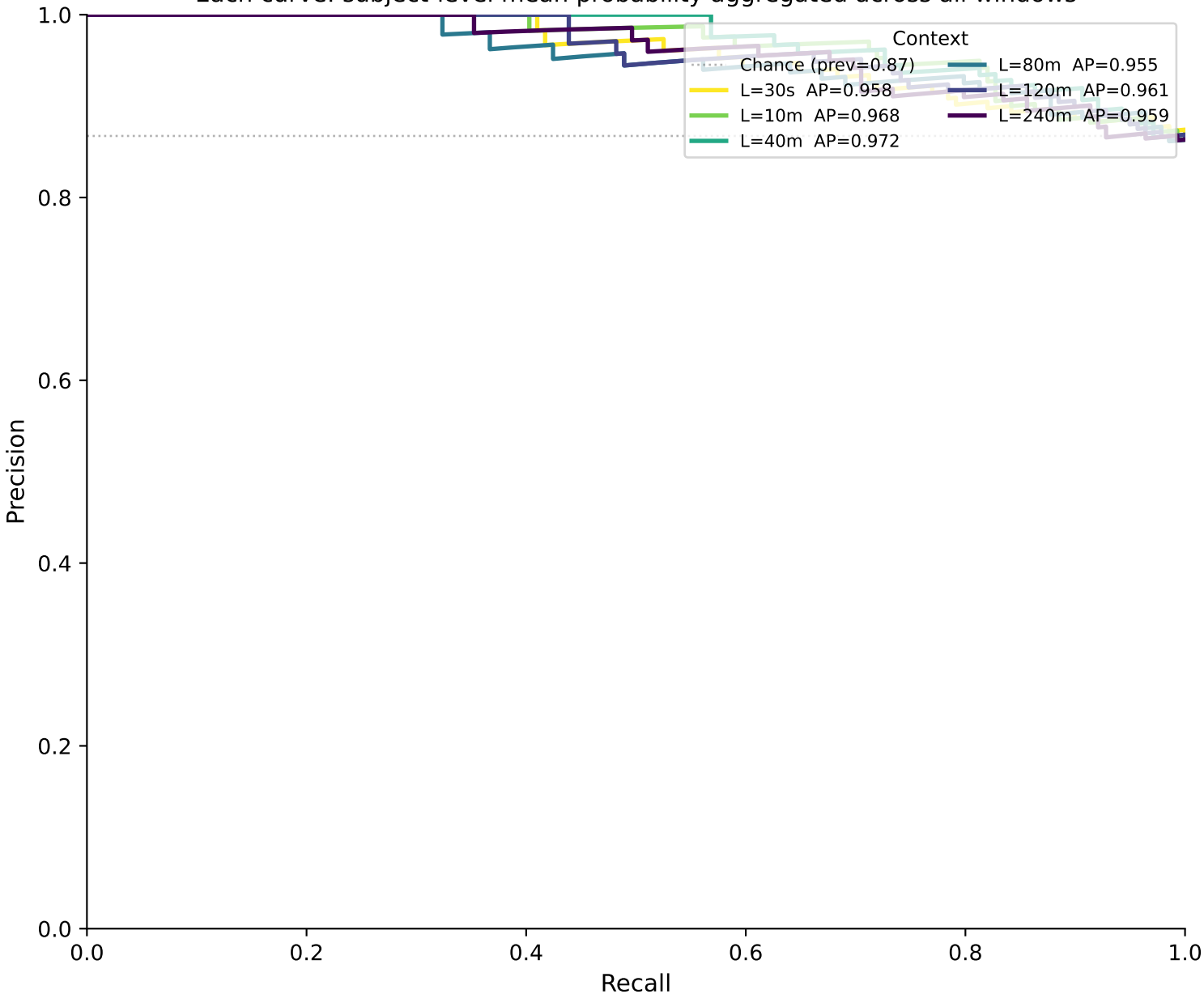
Precision-Recall Curves — osa_binary_apples_postqc (LSTM) K=all Each curve: subject-level mean probability aggregated across all windows
