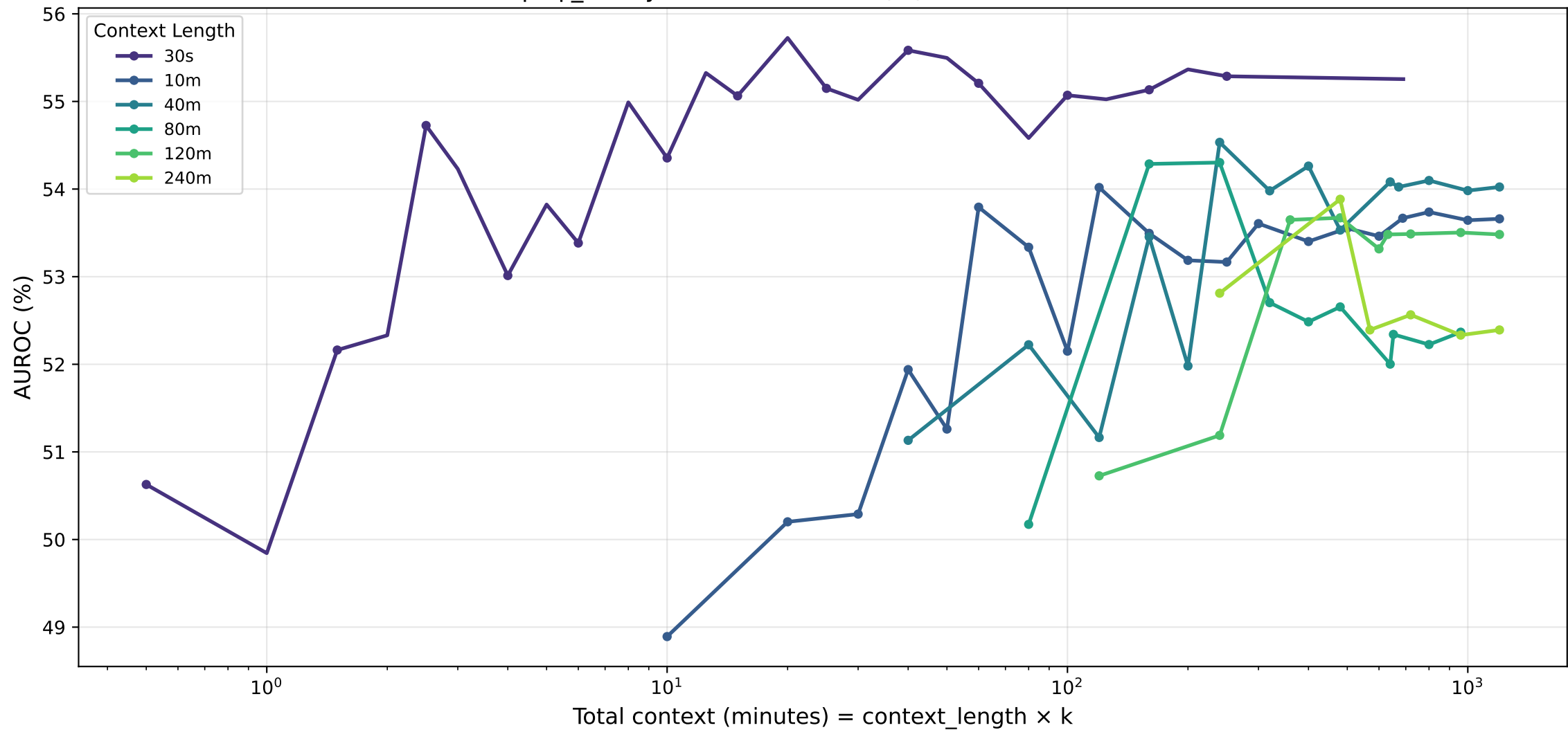
psqi_binary · lstm — AUROC (%) vs Total Context
