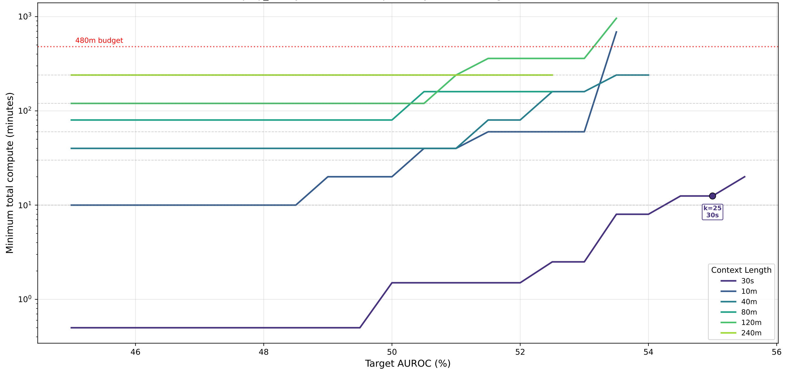
psqi_binary · lstm — Cheapest Way to Reach Target AUROC (%)
