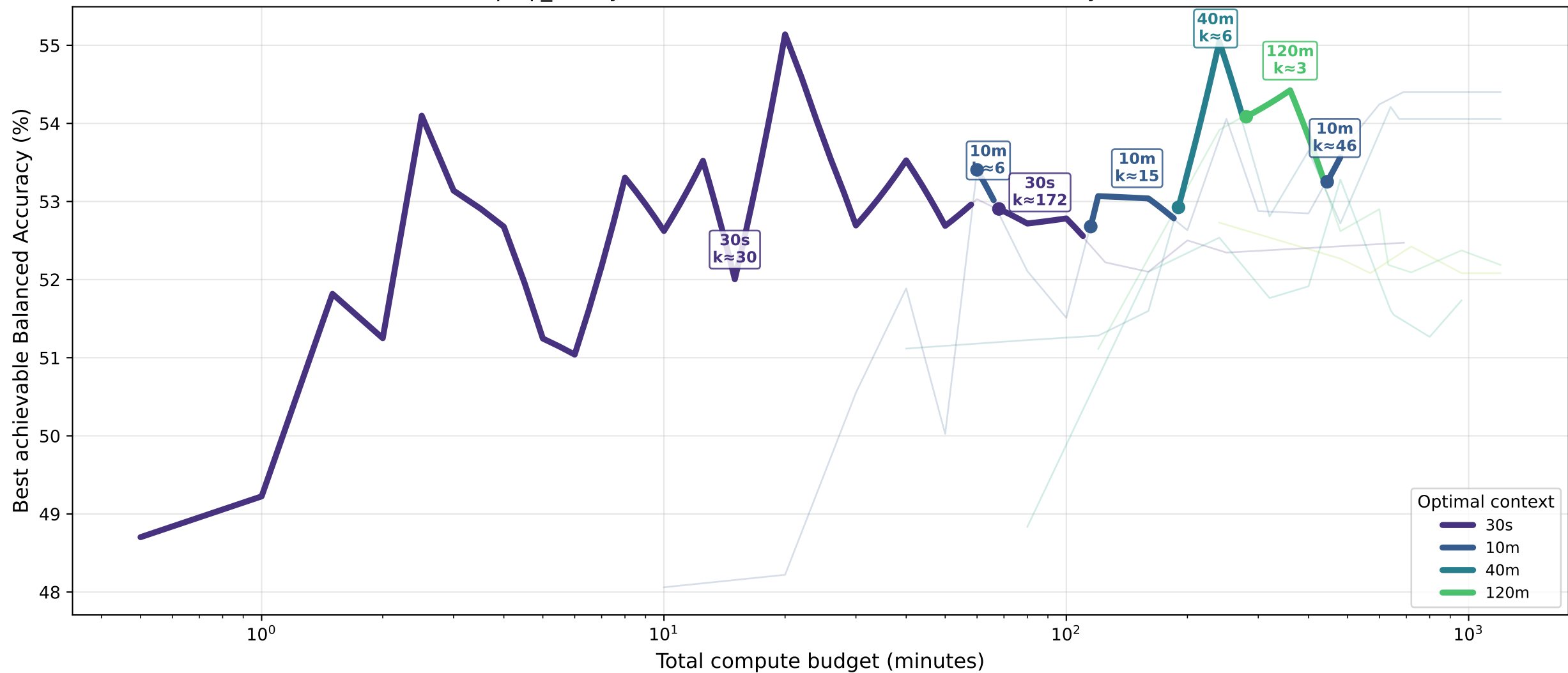
psqi_binary · lstm — Pareto Front: Balanced Accuracy (%)
