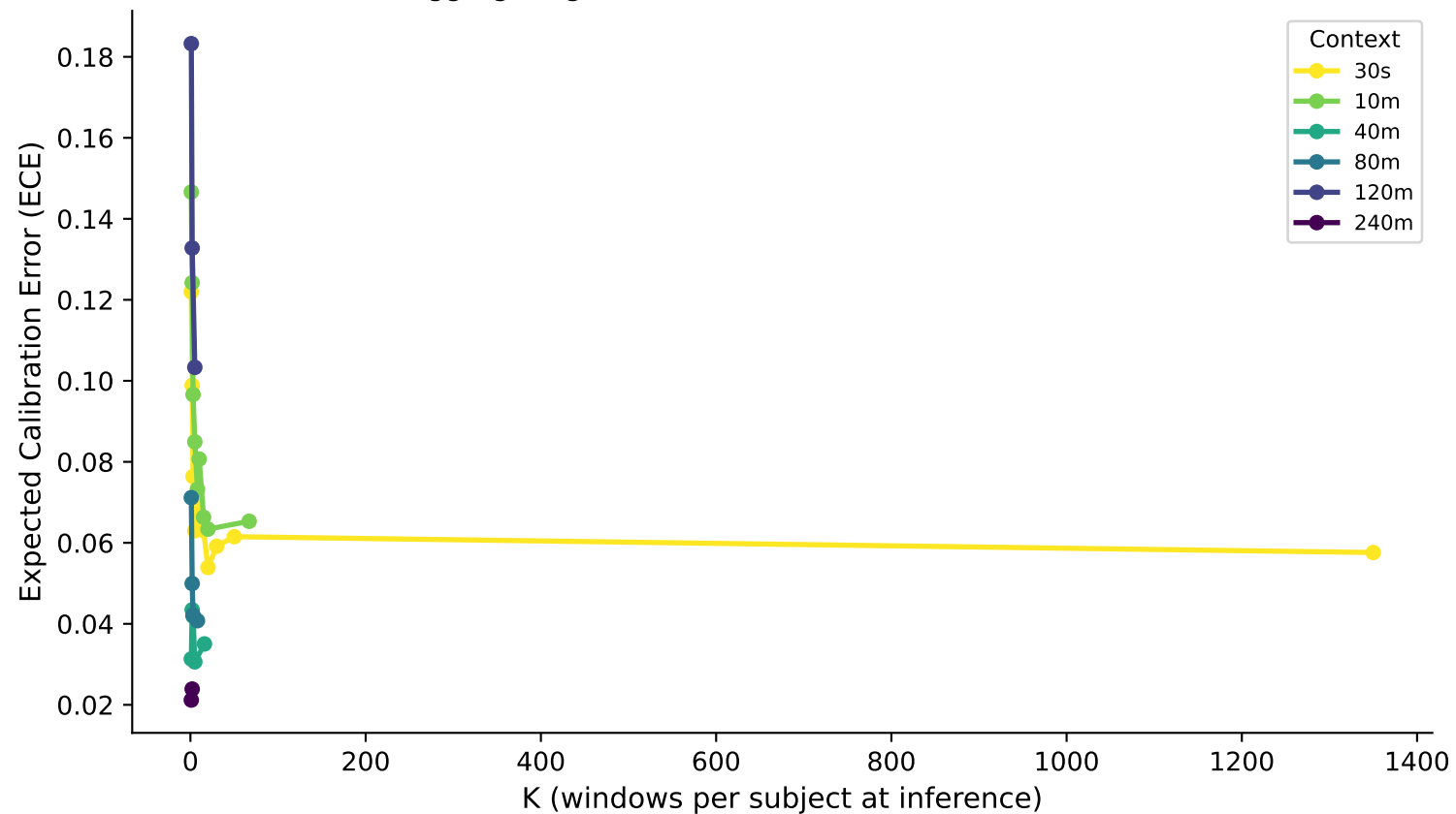
ECE vs K — psqi_binary (LSTM) Aggregating more windows reduces calibration error
